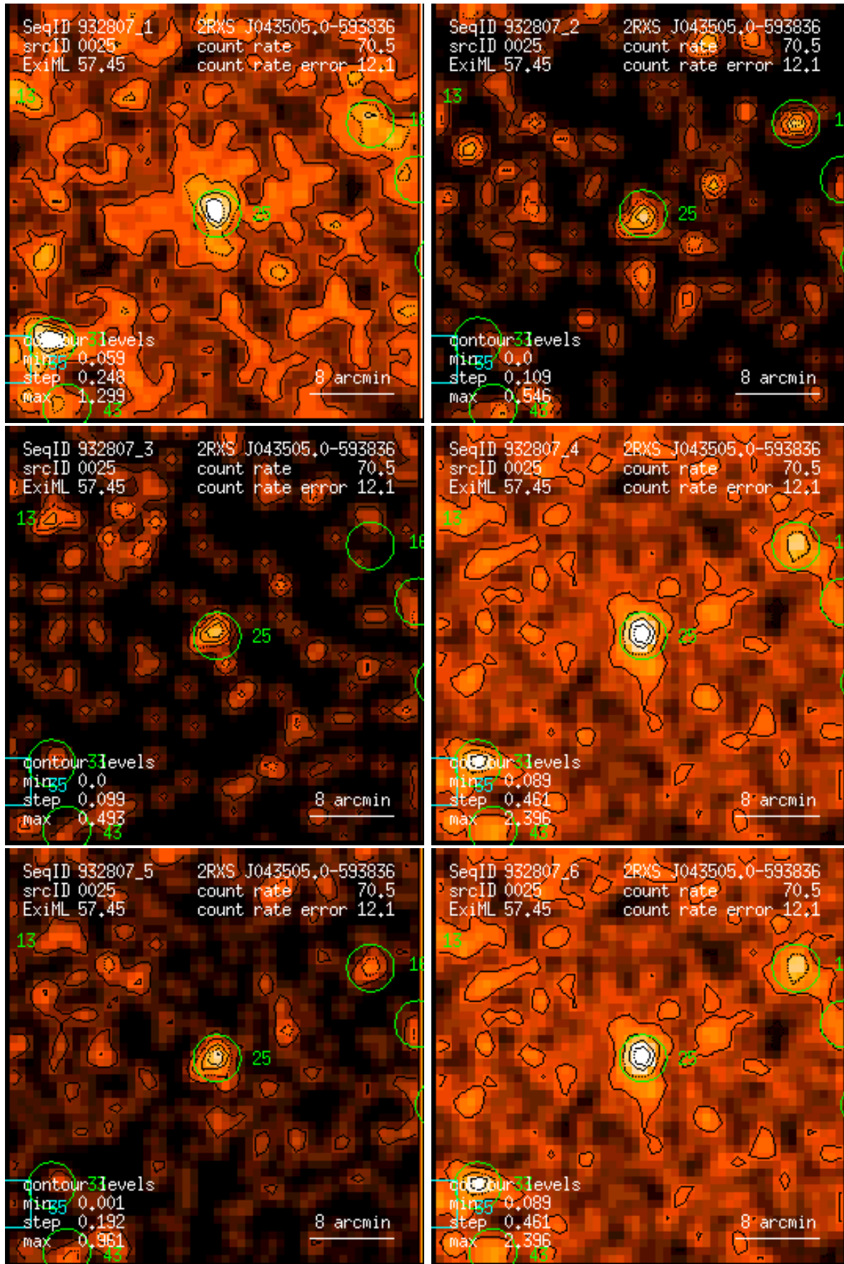
Figure 25: RASS 932807: detection 0025: band rate images, Gaussian filter: (1) PSPC channels 11 – 41, (2) 52 – 90, (3) 91 – 201, (4) 11 – 235, (5) 52 – 201, (6) 11 – 201. Broad band rates in counts/ks. Band rate contour levels in counts/ks/arcmin 2 .
