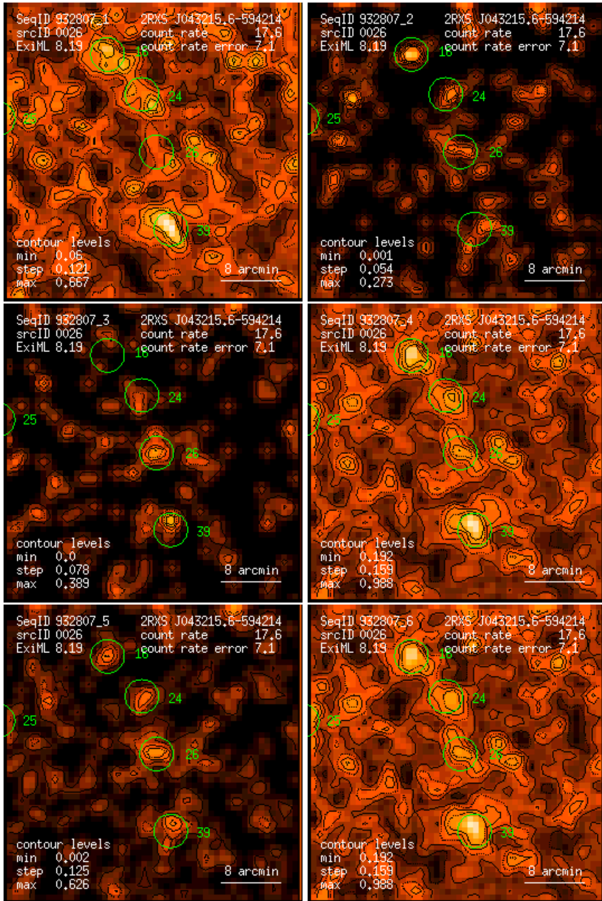
Figure 26: RASS 932807: detection 0026: band rate images, Gaussian filter: (1) PSPC channels 11 – 41, (2) 52 – 90, (3) 91 – 201, (4) 11 – 235, (5) 52 – 201, (6) 11 – 201. Broad band rates in counts/ks. Band rate contour levels in counts/ks/arcmin 2 .
