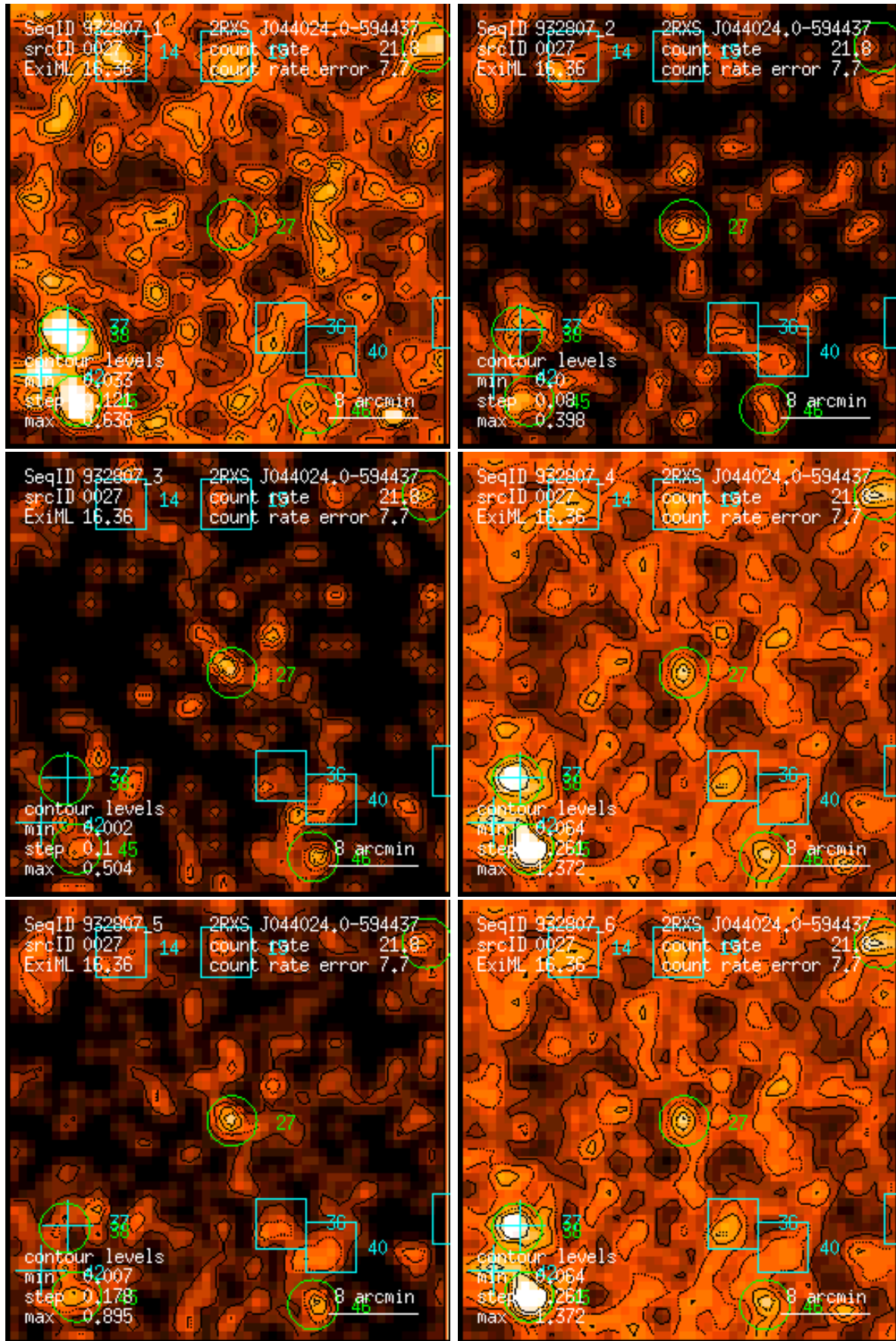
Figure 27: RASS 932807: detection 0027: band rate images, Gaussian filter: (1) PSPC channels 11 – 41, (2) 52 – 90, (3) 91 – 201, (4) 11 – 235, (5) 52 – 201, (6) 11 – 201. Broad band rates in counts/ks. Band rate contour levels in counts/ks/arcmin 2 .
