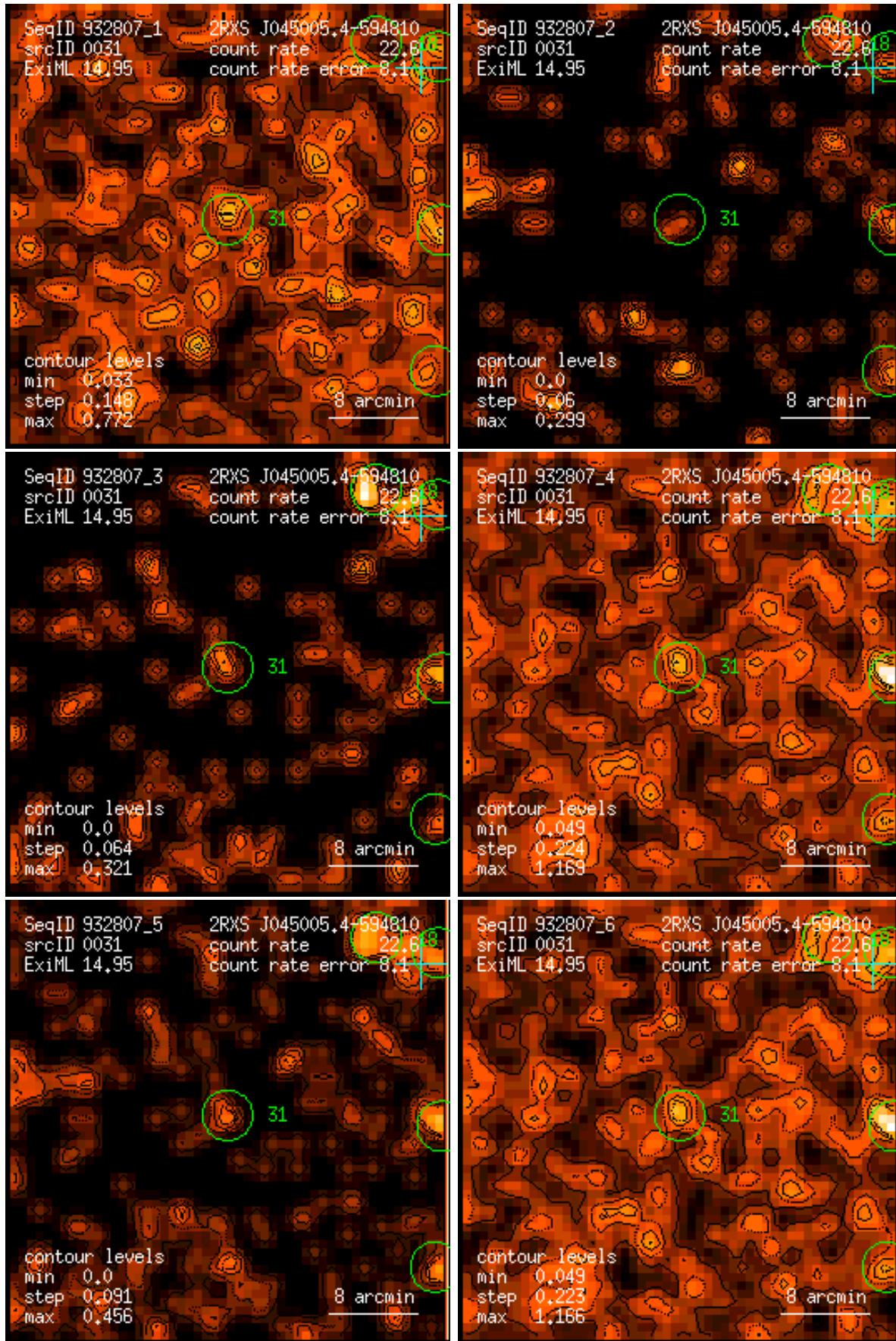
Figure 31: RASS 932807: detection 0031: band rate images, Gaussian filter: (1) PSPC channels 11 – 41, (2) 52 – 90, (3) 91 – 201, (4) 11 – 235, (5) 52 – 201, (6) 11 – 201. Broad band rates in counts/ks. Band rate contour levels in counts/ks/arcmin 2 .
