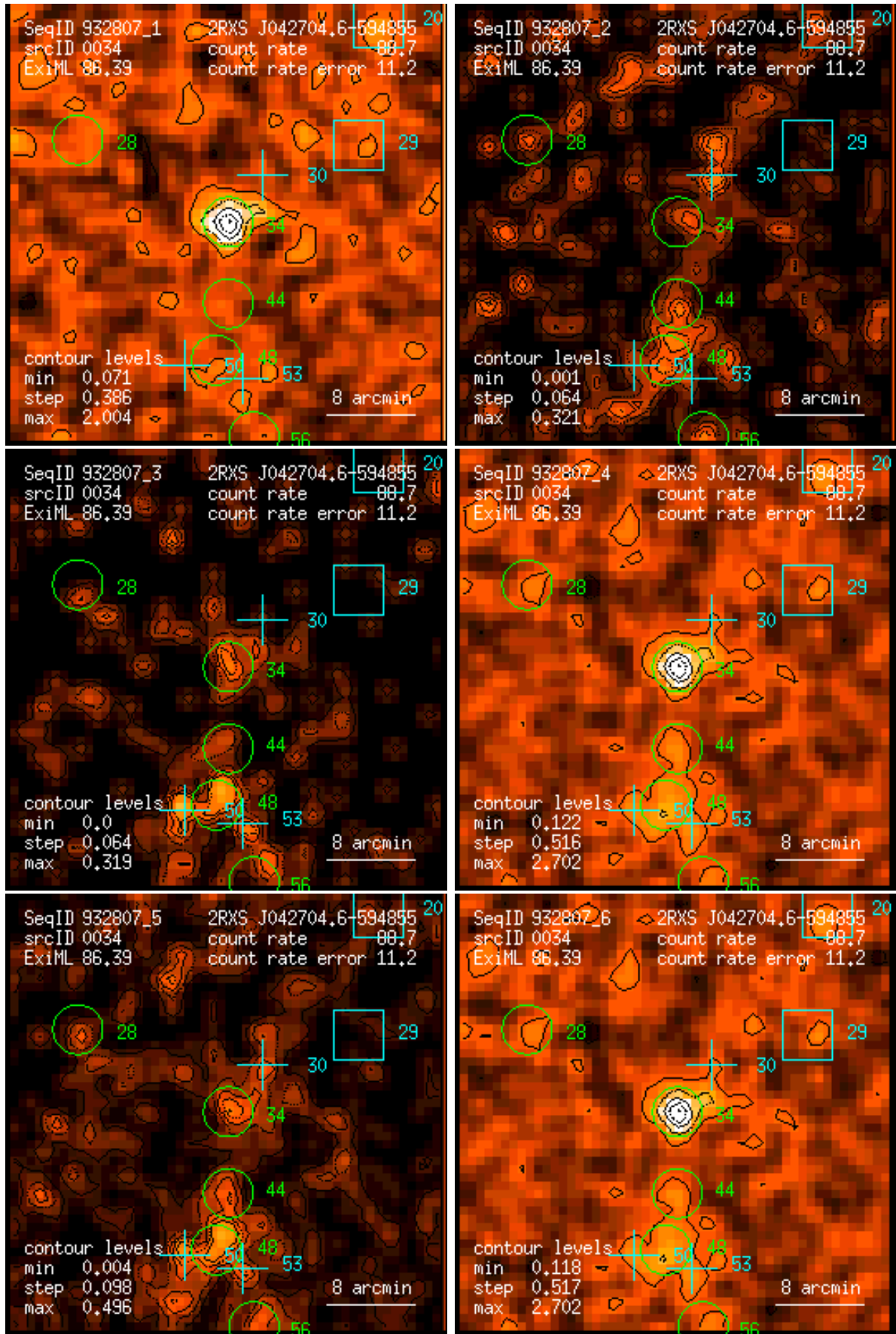
Figure 34: RASS 932807: detection 0034: band rate images, Gaussian filter: (1) PSPC channels 11 – 41, (2) 52 – 90, (3) 91 – 201, (4) 11 – 235, (5) 52 – 201, (6) 11 – 201. Broad band rates in counts/ks. Band rate contour levels in counts/ks/arcmin 2 .
