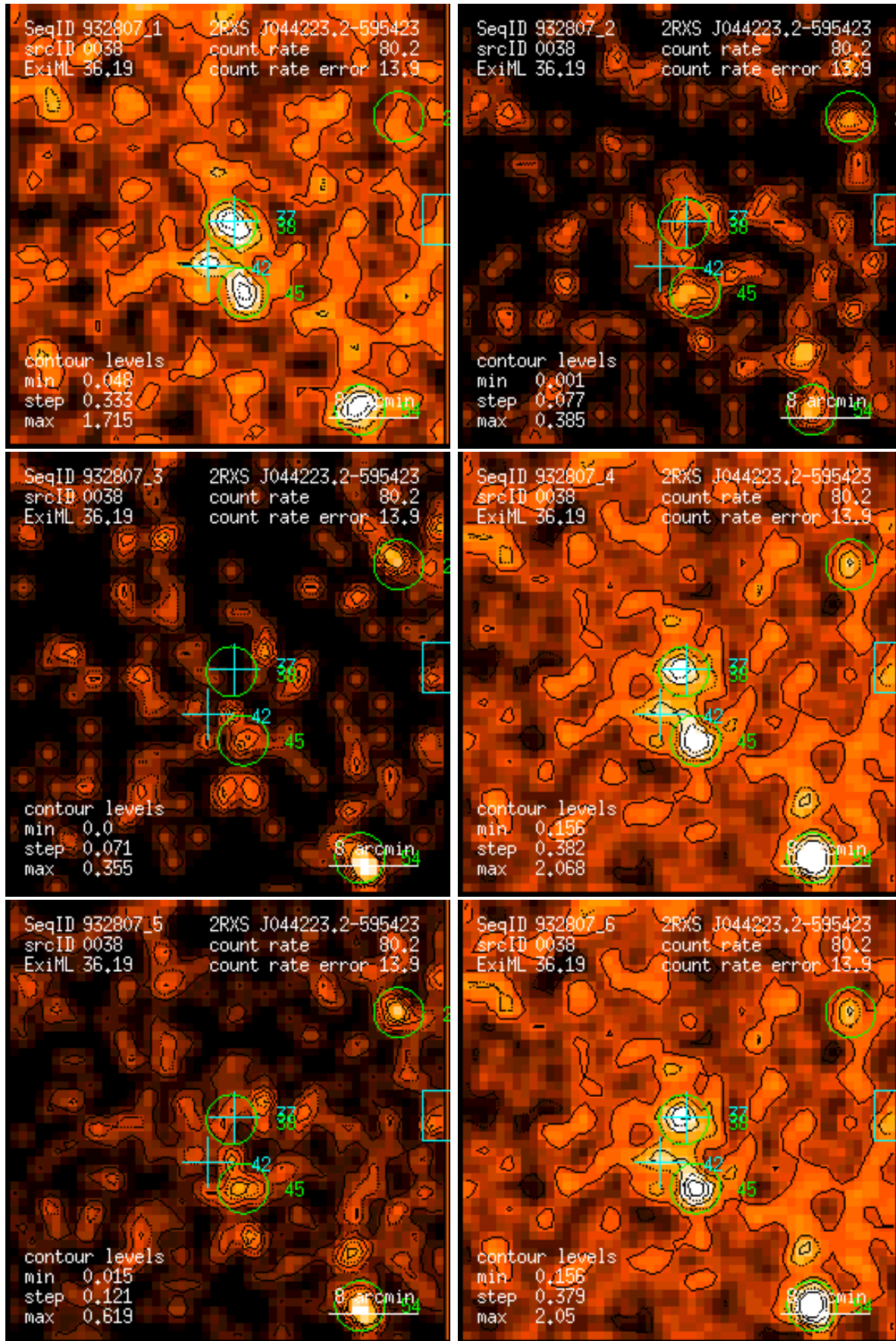
Figure 38: RASS 932807: detection 0038: band rate images, Gaussian filter: (1) PSPC channels 11 – 41, (2) 52 – 90, (3) 91 – 201, (4) 11 – 235, (5) 52 – 201, (6) 11 – 201. Broad band rates in counts/ks. Band rate contour levels in counts/ks/arcmin 2 .
