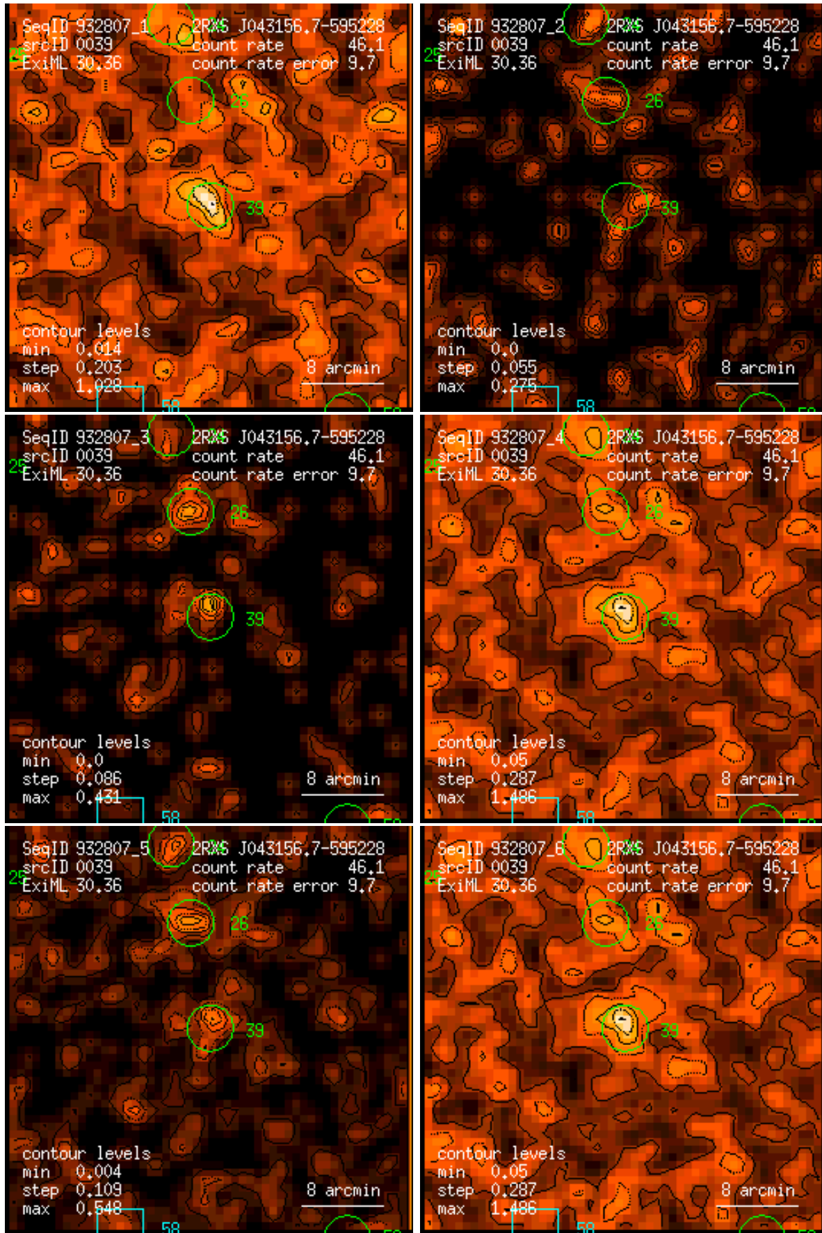
Figure 39: RASS 932807: detection 0039: band rate images, Gaussian filter: (1) PSPC channels 11 – 41, (2) 52 – 90, (3) 91 – 201, (4) 11 – 235, (5) 52 – 201, (6) 11 – 201. Broad band rates in counts/ks. Band rate contour levels in counts/ks/arcmin 2 .
