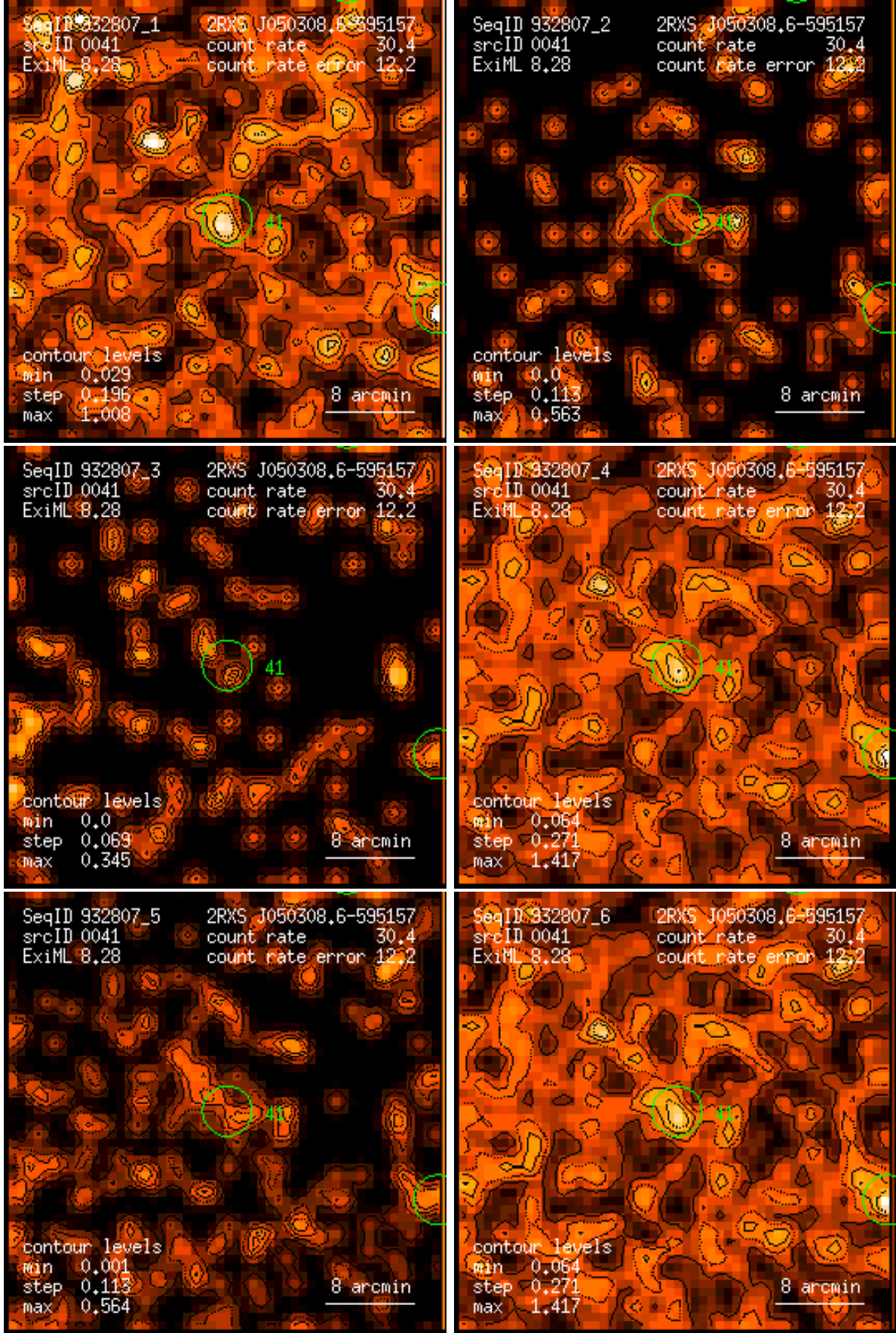
Figure 41: RASS 932807: detection 0041: band rate images, Gaussian filter: (1) PSPC channels 11 – 41, (2) 52 – 90, (3) 91 – 201, (4) 11 – 235, (5) 52 – 201, (6) 11 – 201. Broad band rates in counts/ks. Band rate contour levels in counts/ks/arcmin 2 .
