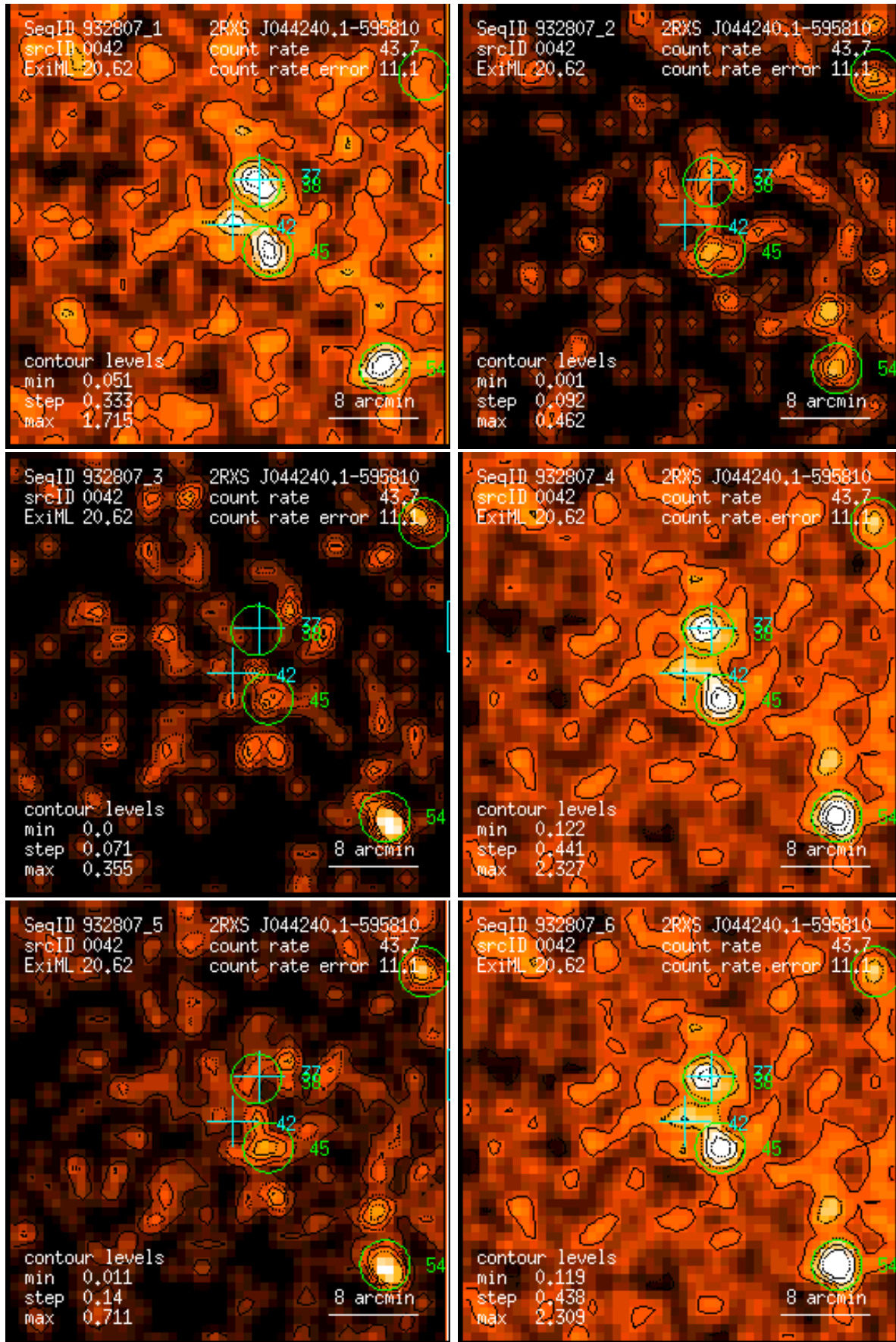
Figure 42: RASS 932807: detection 0042: band rate images, Gaussian filter: (1) PSPC channels 11 – 41, (2) 52 – 90, (3) 91 – 201, (4) 11 – 235, (5) 52 – 201, (6) 11 – 201. Broad band rates in counts/ks. Band rate contour levels in counts/ks/arcmin 2 .
