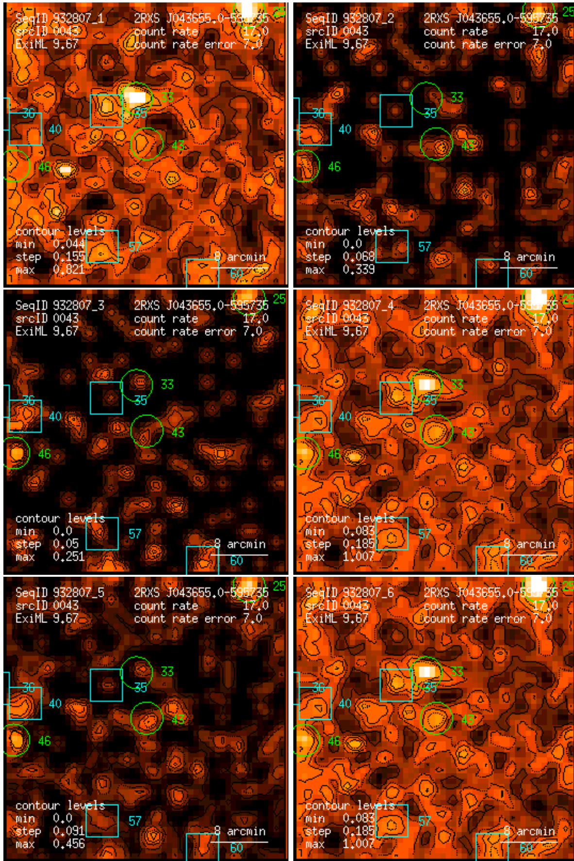
Figure 43: RASS 932807: detection 0043: band rate images, Gaussian filter: (1) PSPC channels 11 – 41, (2) 52 – 90, (3) 91 – 201, (4) 11 – 235, (5) 52 – 201, (6) 11 – 201. Broad band rates in counts/ks. Band rate contour levels in counts/ks/arcmin 2 .
