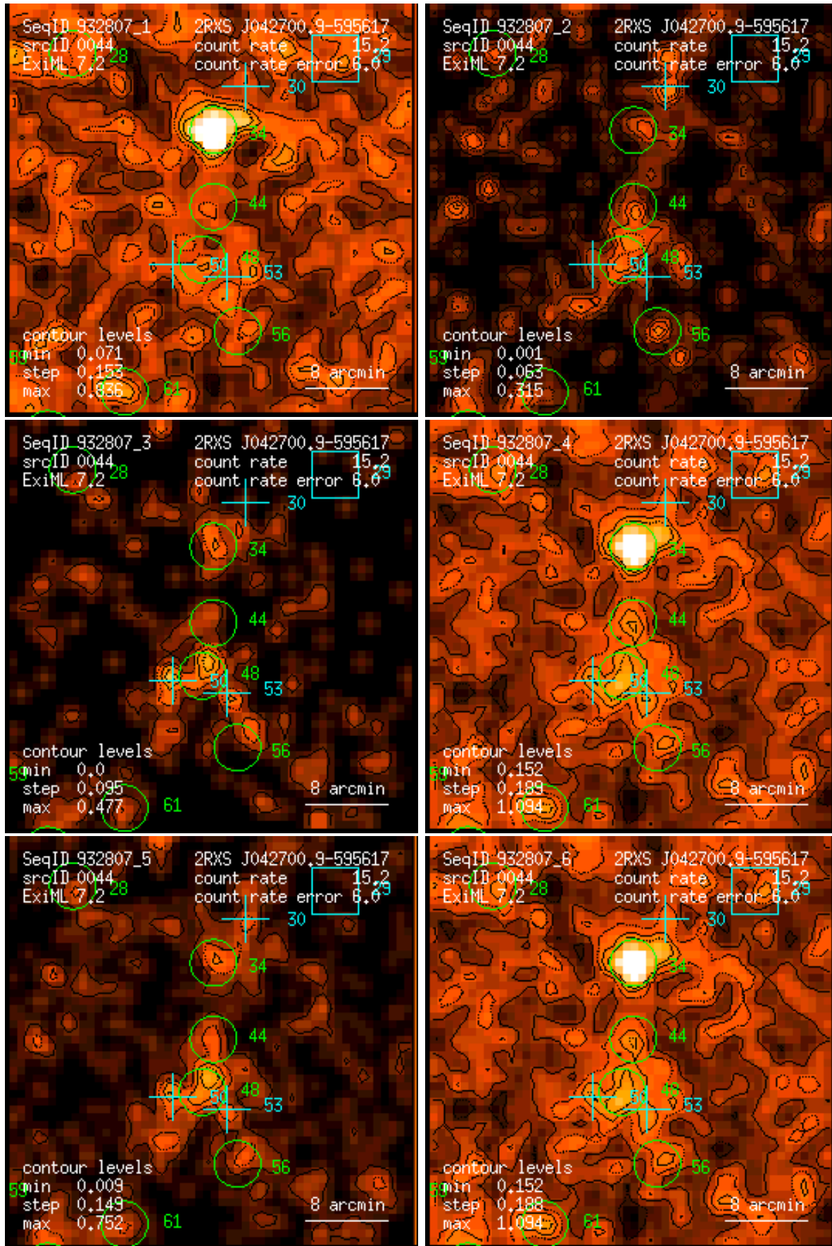
Figure 44: RASS 932807: detection 0044: band rate images, Gaussian filter: (1) PSPC channels 11 – 41, (2) 52 – 90, (3) 91 – 201, (4) 11 – 235, (5) 52 – 201, (6) 11 – 201. Broad band rates in counts/ks. Band rate contour levels in counts/ks/arcmin 2 .
