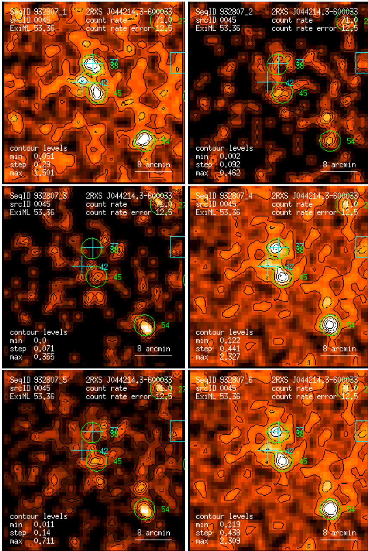
Figure 45: RASS 932807: detection 0045: band rate images, Gaussian filter: (1) PSPC channels 11 – 41, (2) 52 – 90, (3) 91 – 201, (4) 11 – 235, (5) 52 – 201, (6) 11 – 201. Broad band rates in counts/ks. Band rate contour levels in counts/ks/arcmin 2 .
