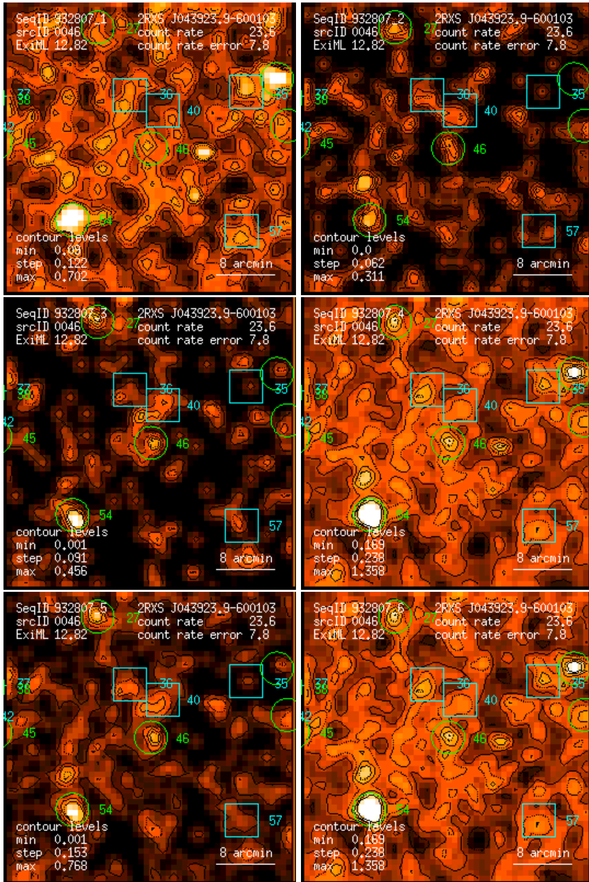
Figure 46: RASS 932807: detection 0046: band rate images, Gaussian filter: (1) PSPC channels 11 – 41, (2) 52 – 90, (3) 91 – 201, (4) 11 – 235, (5) 52 – 201, (6) 11 – 201. Broad band rates in counts/ks. Band rate contour levels in counts/ks/arcmin 2 .
