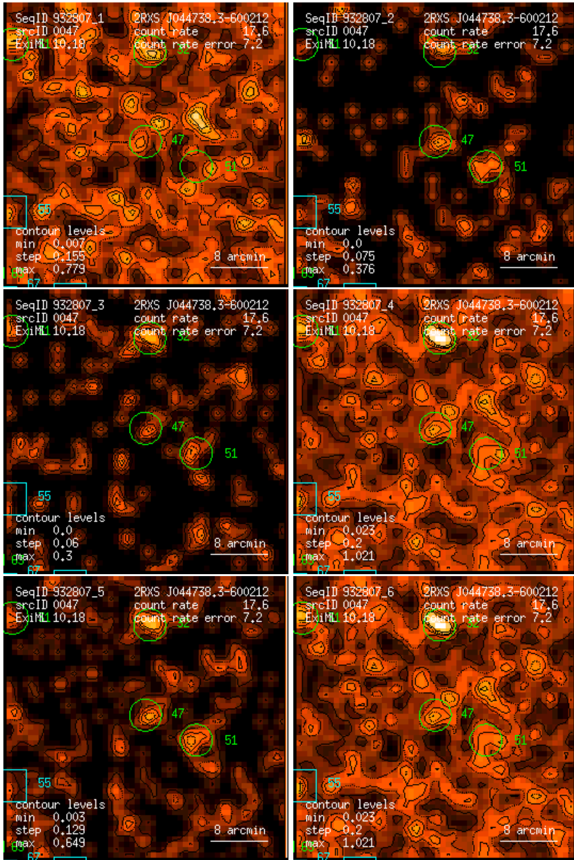
Figure 47: RASS 932807: detection 0047: band rate images, Gaussian filter: (1) PSPC channels 11 – 41, (2) 52 – 90, (3) 91 – 201, (4) 11 – 235, (5) 52 – 201, (6) 11 – 201. Broad band rates in counts/ks. Band rate contour levels in counts/ks/arcmin 2 .
