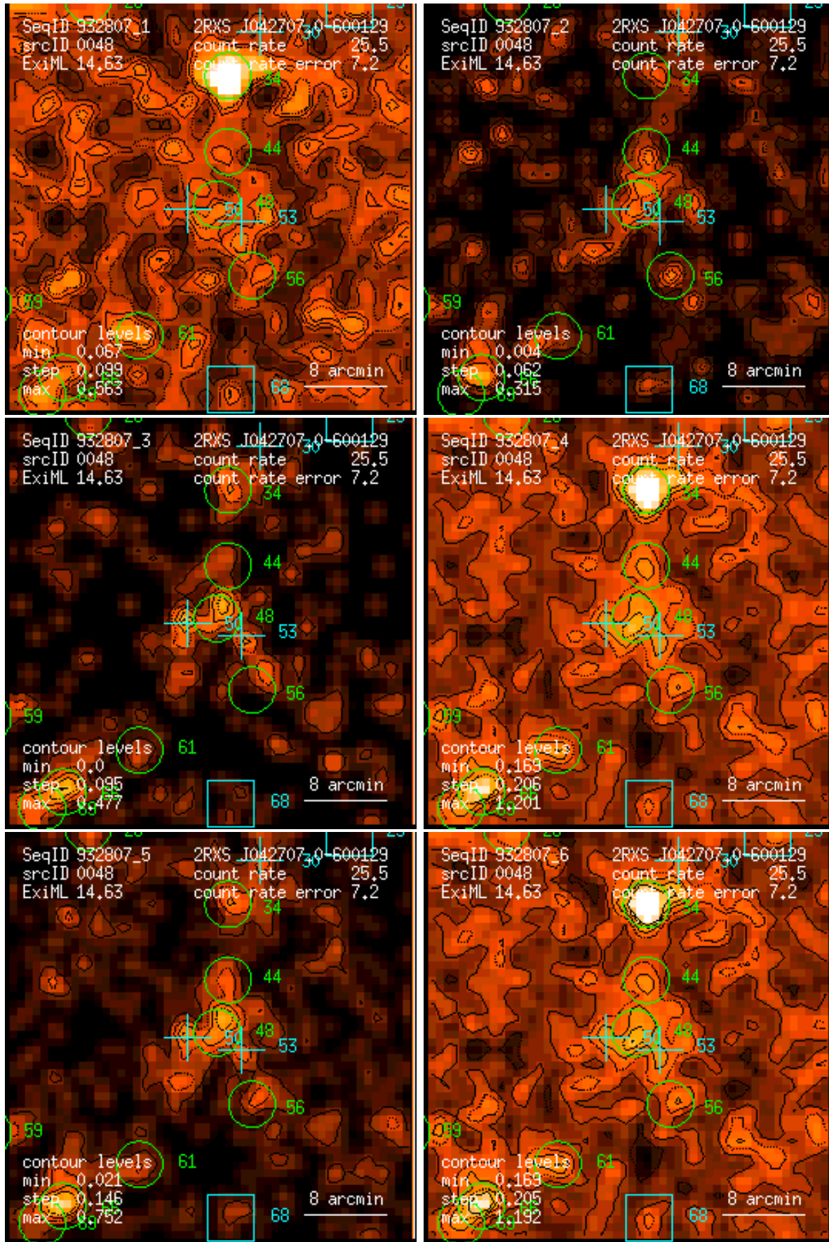
Figure 48: RASS 932807: detection 0048: band rate images, Gaussian filter: (1) PSPC channels 11 – 41, (2) 52 – 90, (3) 91 – 201, (4) 11 – 235, (5) 52 – 201, (6) 11 – 201. Broad band rates in counts/ks. Band rate contour levels in counts/ks/arcmin 2 .
