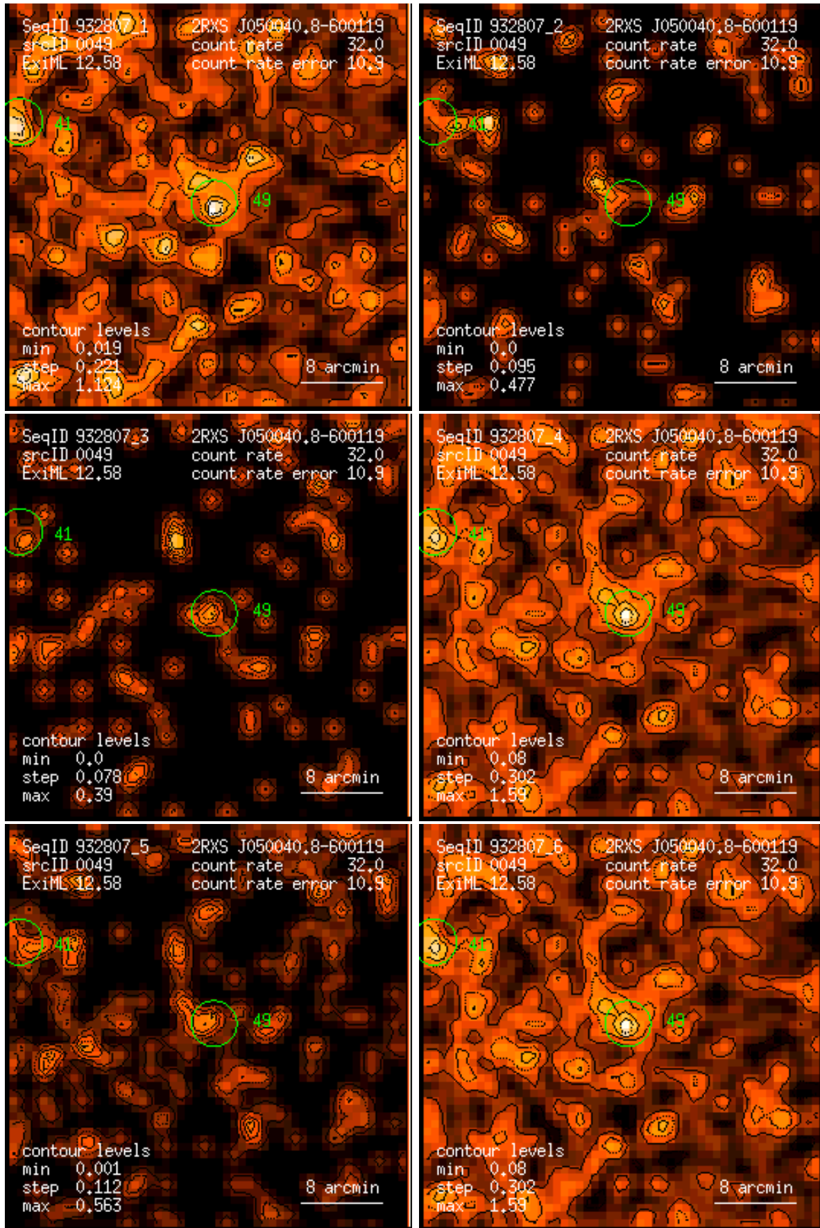
Figure 49: RASS 932807: detection 0049: band rate images, Gaussian filter: (1) PSPC channels 11 – 41, (2) 52 – 90, (3) 91 – 201, (4) 11 – 235, (5) 52 – 201, (6) 11 – 201. Broad band rates in counts/ks. Band rate contour levels in counts/ks/arcmin 2 .
