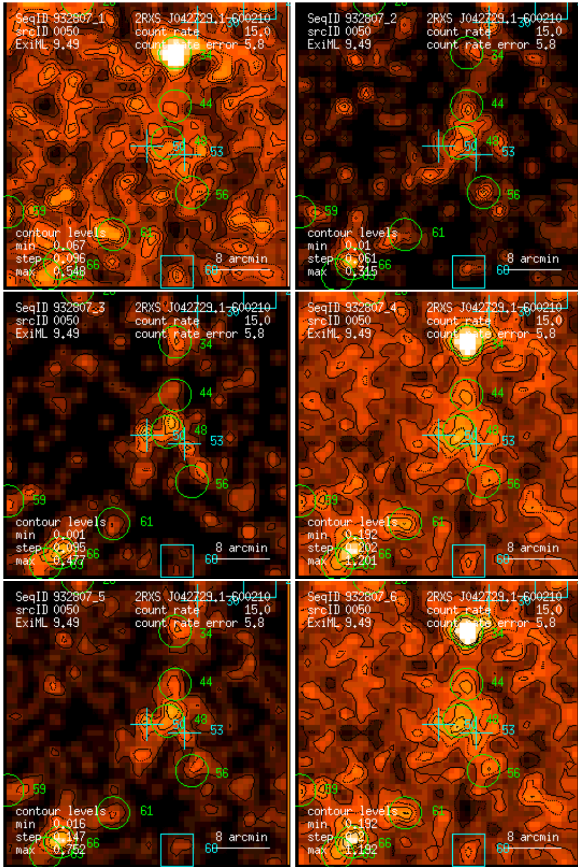
Figure 50: RASS 932807: detection 0050: band rate images, Gaussian filter: (1) PSPC channels 11 – 41, (2) 52 – 90, (3) 91 – 201, (4) 11 – 235, (5) 52 – 201, (6) 11 – 201. Broad band rates in counts/ks. Band rate contour levels in counts/ks/arcmin 2 .
