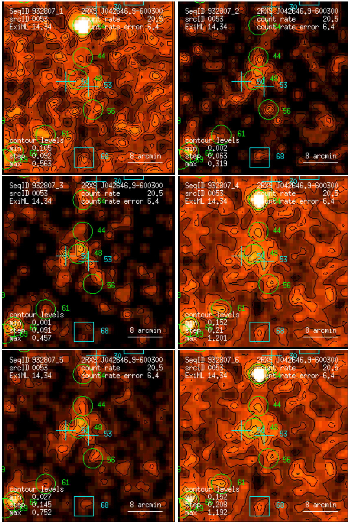
Figure 53: RASS 932807: detection 0053: band rate images, Gaussian filter: (1) PSPC channels 11 – 41, (2) 52 – 90, (3) 91 – 201, (4) 11 – 235, (5) 52 – 201, (6) 11 – 201. Broad band rates in counts/ks. Band rate contour levels in counts/ks/arcmin 2 .
