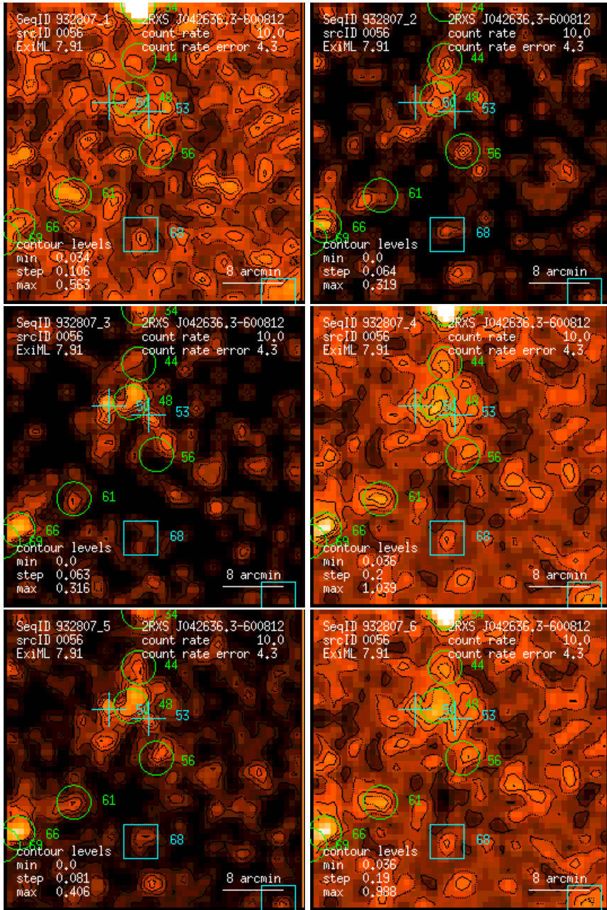
Figure 56: RASS 932807: detection 0056: band rate images, Gaussian filter: (1) PSPC channels 11 – 41, (2) 52 – 90, (3) 91 – 201, (4) 11 – 235, (5) 52 – 201, (6) 11 – 201. Broad band rates in counts/ks. Band rate contour levels in counts/ks/arcmin 2 .
