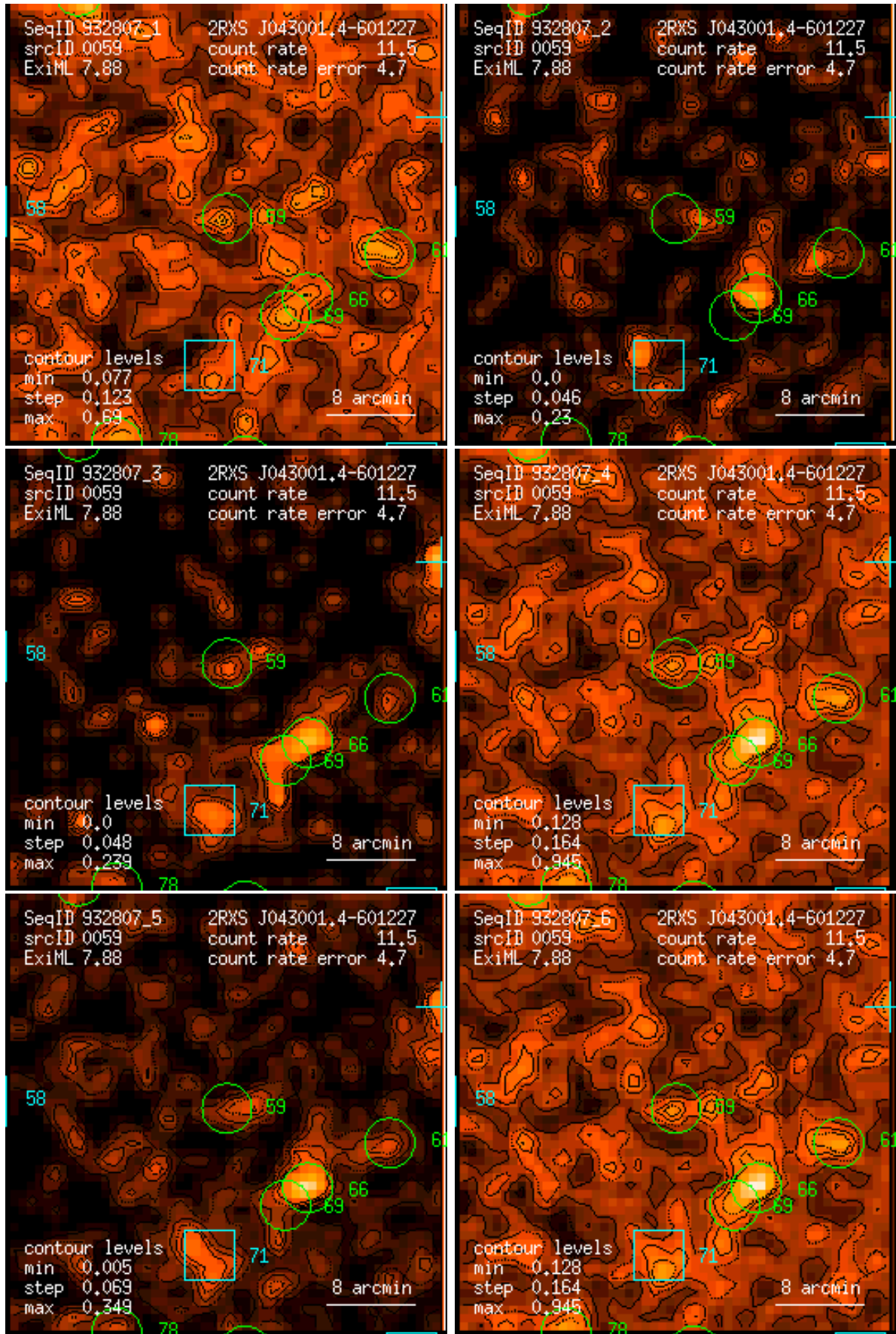
Figure 59: RASS 932807: detection 0059: band rate images, Gaussian filter: (1) PSPC channels 11 – 41, (2) 52 – 90, (3) 91 – 201, (4) 11 – 235, (5) 52 – 201, (6) 11 – 201. Broad band rates in counts/ks. Band rate contour levels in counts/ks/arcmin 2 .
