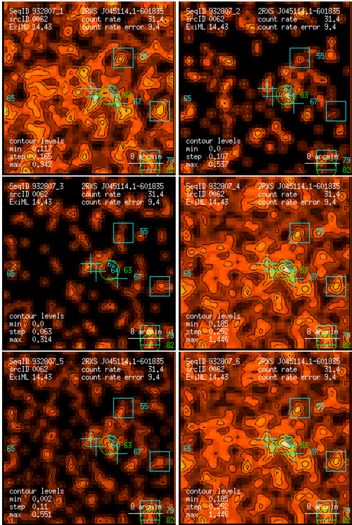
Figure 62: RASS 932807: detection 0062: band rate images, Gaussian filter: (1) PSPC channels 11 – 41, (2) 52 – 90, (3) 91 – 201, (4) 11 – 235, (5) 52 – 201, (6) 11 – 201. Broad band rates in counts/ks. Band rate contour levels in counts/ks/arcmin 2 .
