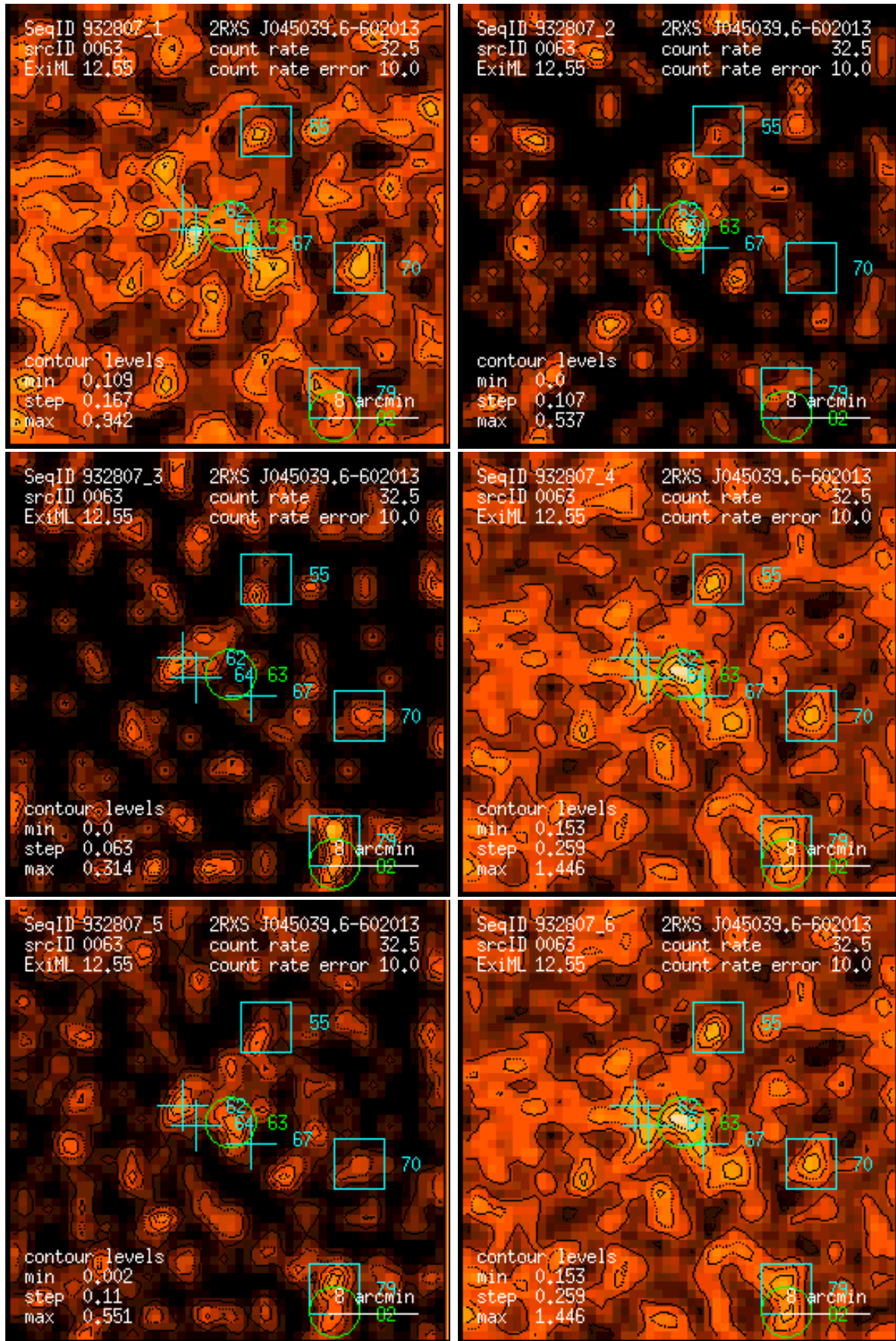
Figure 63: RASS 932807: detection 0063: band rate images, Gaussian filter: (1) PSPC channels 11 – 41, (2) 52 – 90, (3) 91 – 201, (4) 11 – 235, (5) 52 – 201, (6) 11 – 201. Broad band rates in counts/ks. Band rate contour levels in counts/ks/arcmin 2 .
