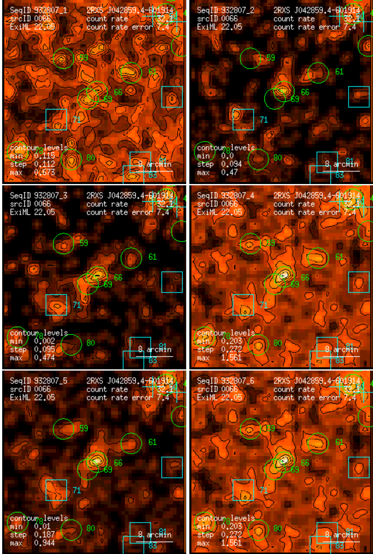
Figure 66: RASS 932807: detection 0066: band rate images, Gaussian filter: (1) PSPC channels 11 – 41, (2) 52 – 90, (3) 91 – 201, (4) 11 – 235, (5) 52 – 201, (6) 11 – 201. Broad band rates in counts/ks. Band rate contour levels in counts/ks/arcmin 2 .
