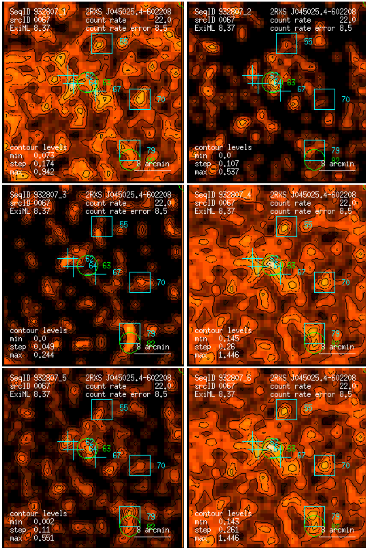
Figure 67: RASS 932807: detection 0067: band rate images, Gaussian filter: (1) PSPC channels 11 – 41, (2) 52 – 90, (3) 91 – 201, (4) 11 – 235, (5) 52 – 201, (6) 11 – 201. Broad band rates in counts/ks. Band rate contour levels in counts/ks/arcmin 2 .
