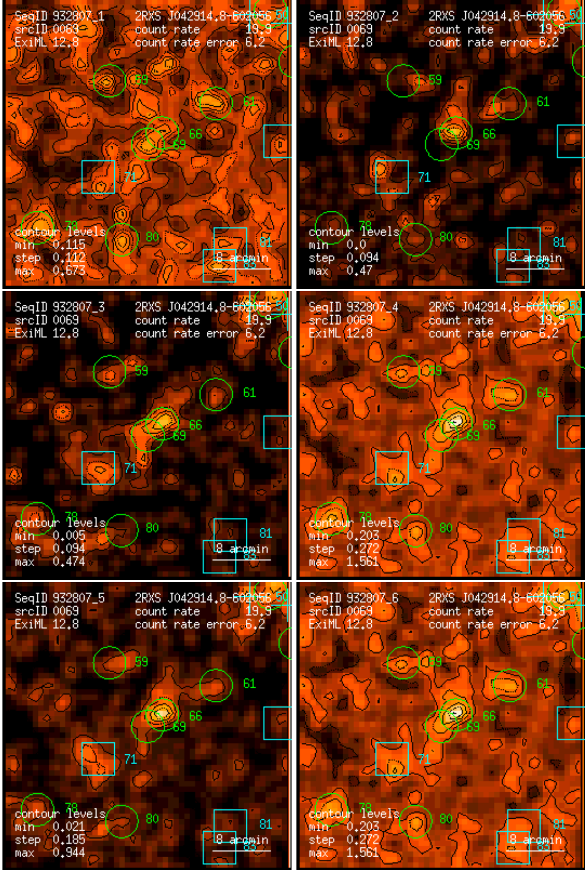
Figure 69: RASS 932807: detection 0069: band rate images, Gaussian filter: (1) PSPC channels 11 – 41, (2) 52 – 90, (3) 91 – 201, (4) 11 – 235, (5) 52 – 201, (6) 11 – 201. Broad band rates in counts/ks. Band rate contour levels in counts/ks/arcmin 2 .
