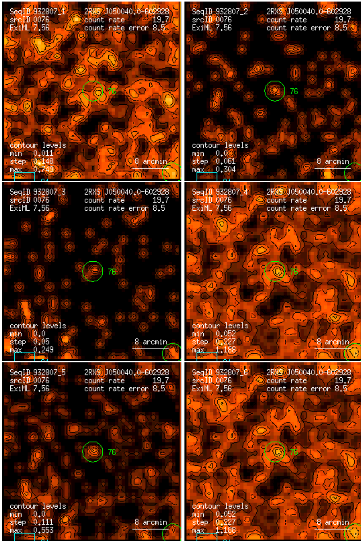
Figure 76: RASS 932807: detection 0076: band rate images, Gaussian filter: (1) PSPC channels 11 – 41, (2) 52 – 90, (3) 91 – 201, (4) 11 – 235, (5) 52 – 201, (6) 11 – 201. Broad band rates in counts/ks. Band rate contour levels in counts/ks/arcmin 2 .
