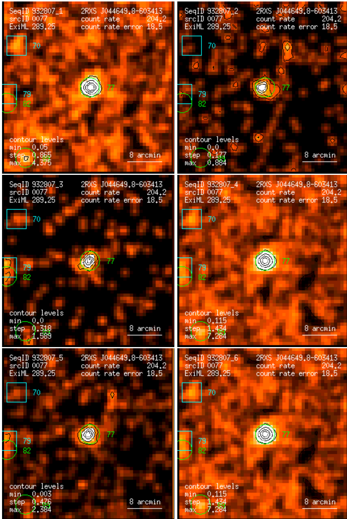
Figure 77: RASS 932807: detection 0077: band rate images, Gaussian filter: (1) PSPC channels 11 – 41, (2) 52 – 90, (3) 91 – 201, (4) 11 – 235, (5) 52 – 201, (6) 11 – 201. Broad band rates in counts/ks. Band rate contour levels in counts/ks/arcmin 2 .
