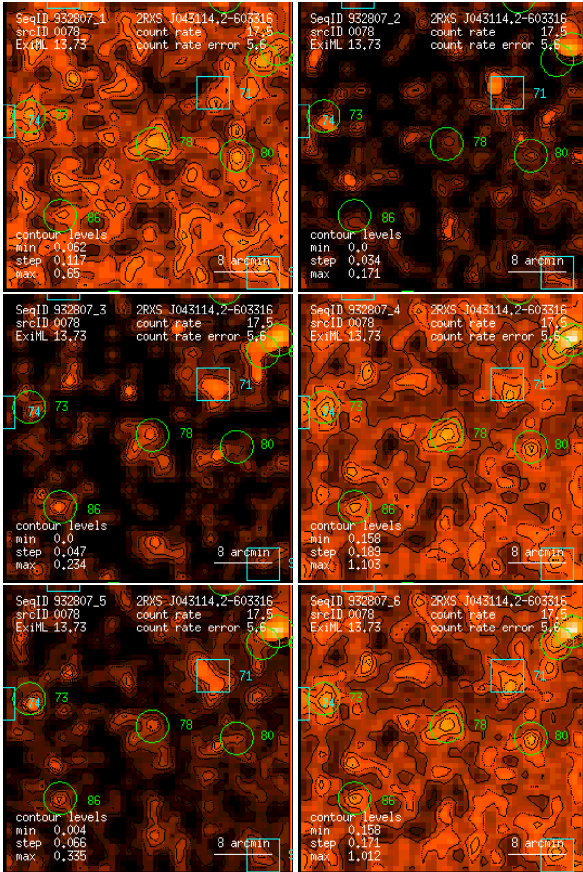
Figure 78: RASS 932807: detection 0078: band rate images, Gaussian filter: (1) PSPC channels 11 – 41, (2) 52 – 90, (3) 91 – 201, (4) 11 – 235, (5) 52 – 201, (6) 11 – 201. Broad band rates in counts/ks. Band rate contour levels in counts/ks/arcmin 2 .
