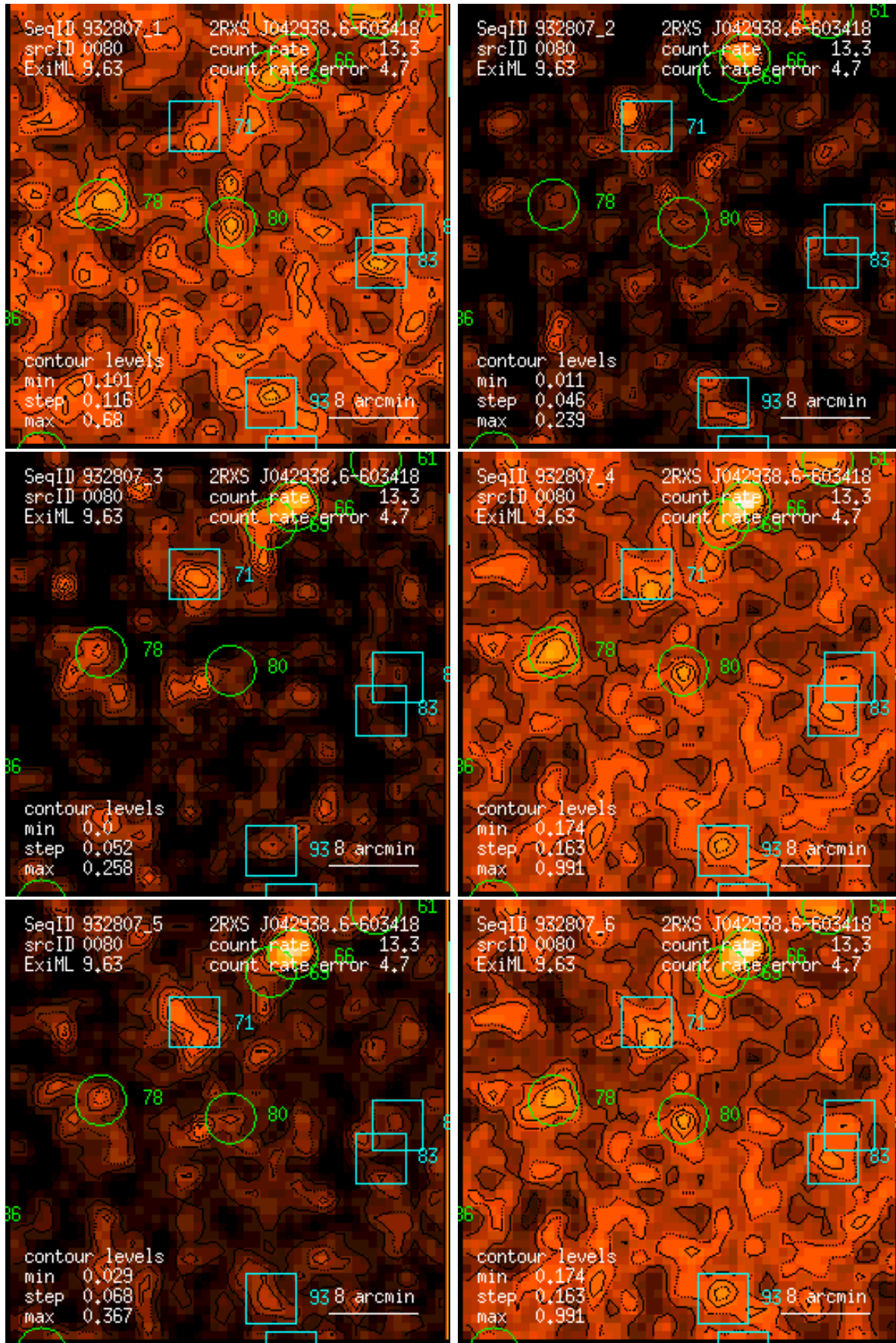
Figure 80: RASS 932807: detection 0080: band rate images, Gaussian filter: (1) PSPC channels 11 – 41, (2) 52 – 90, (3) 91 – 201, (4) 11 – 235, (5) 52 – 201, (6) 11 – 201. Broad band rates in counts/ks. Band rate contour levels in counts/ks/arcmin 2 .
