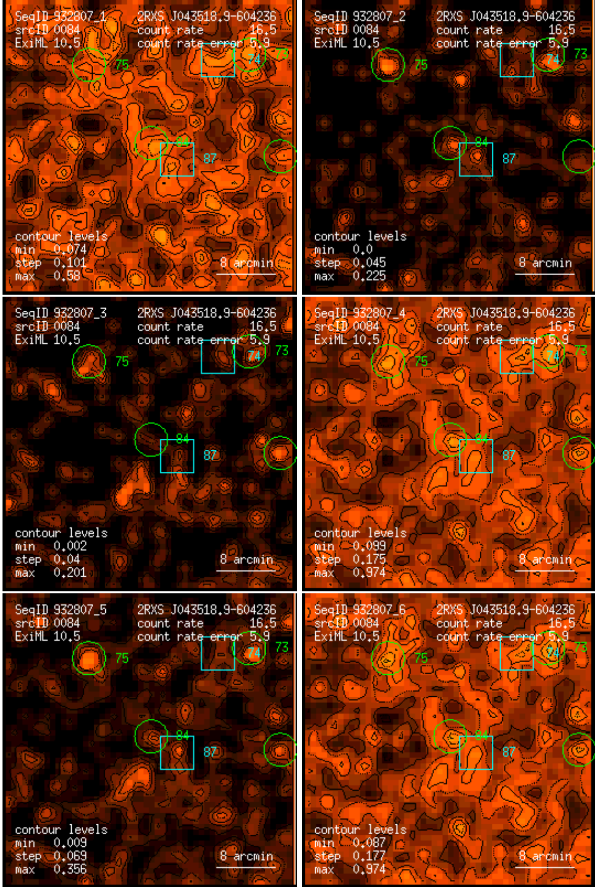
Figure 84: RASS 932807: detection 0084: band rate images, Gaussian filter: (1) PSPC channels 11 – 41, (2) 52 – 90, (3) 91 – 201, (4) 11 – 235, (5) 52 – 201, (6) 11 – 201. Broad band rates in counts/ks. Band rate contour levels in counts/ks/arcmin 2 .
