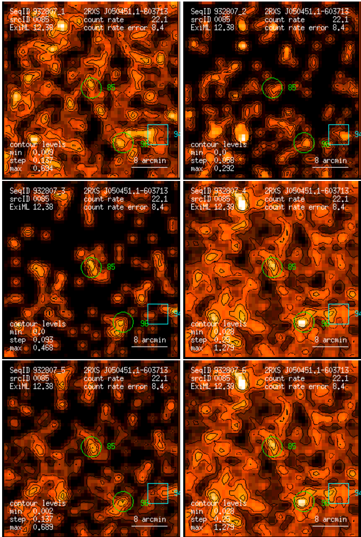
Figure 85: RASS 932807: detection 0085: band rate images, Gaussian filter: (1) PSPC channels 11 – 41, (2) 52 – 90, (3) 91 – 201, (4) 11 – 235, (5) 52 – 201, (6) 11 – 201. Broad band rates in counts/ks. Band rate contour levels in counts/ks/arcmin 2 .
