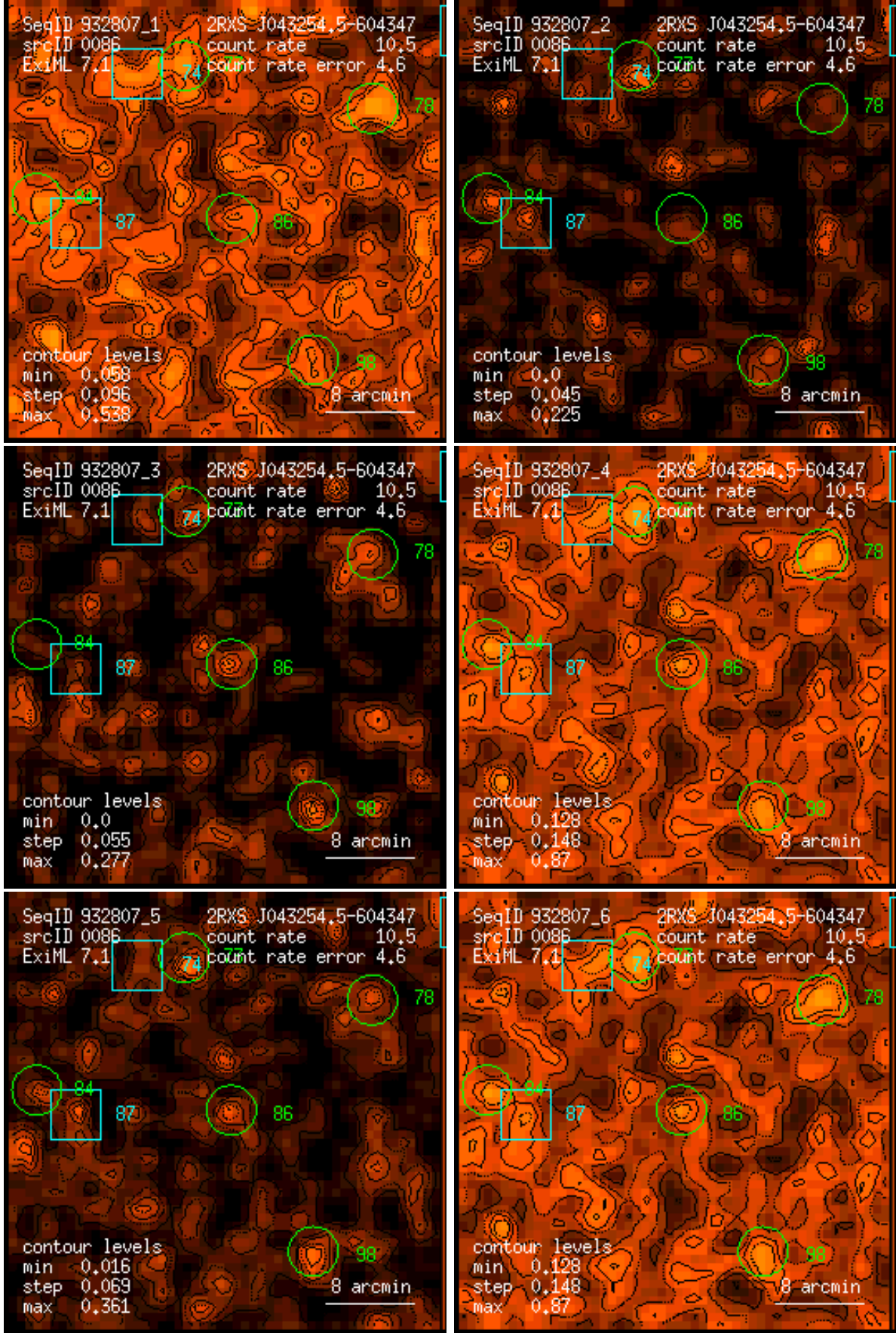
Figure 86: RASS 932807: detection 0086: band rate images, Gaussian filter: (1) PSPC channels 11 – 41, (2) 52 – 90, (3) 91 – 201, (4) 11 – 235, (5) 52 – 201, (6) 11 – 201. Broad band rates in counts/ks. Band rate contour levels in counts/ks/arcmin 2 .
