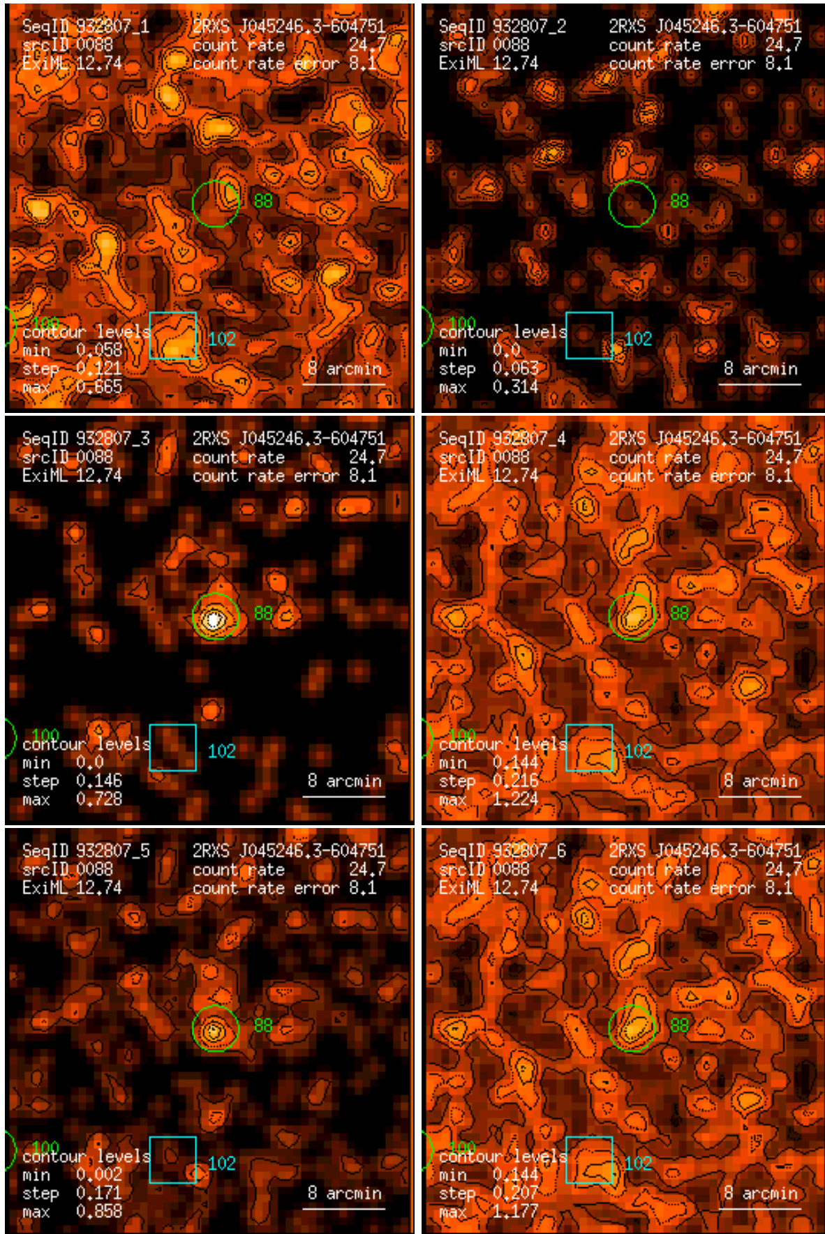
Figure 88: RASS 932807: detection 0088: band rate images, Gaussian filter: (1) PSPC channels 11 – 41, (2) 52 – 90, (3) 91 – 201, (4) 11 – 235, (5) 52 – 201, (6) 11 – 201. Broad band rates in counts/ks. Band rate contour levels in counts/ks/arcmin 2 .
