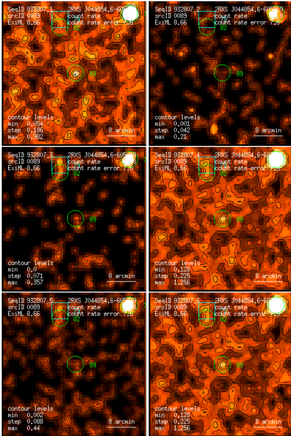
Figure 89: RASS 932807: detection 0089: band rate images, Gaussian filter: (1) PSPC channels 11 – 41, (2) 52 – 90, (3) 91 – 201, (4) 11 – 235, (5) 52 – 201, (6) 11 – 201. Broad band rates in counts/ks. Band rate contour levels in counts/ks/arcmin 2 .
