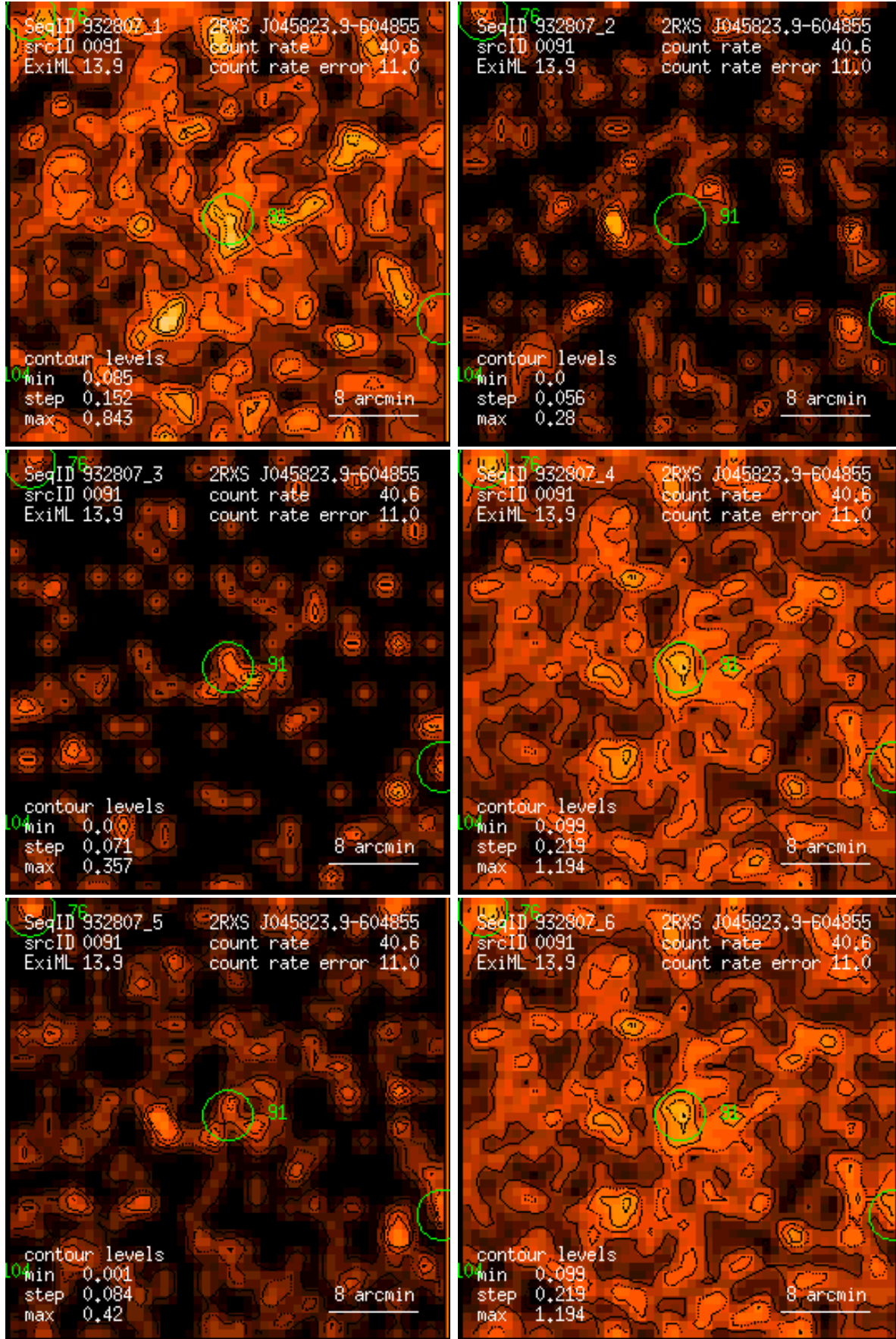
Figure 91: RASS 932807: detection 0091: band rate images, Gaussian filter: (1) PSPC channels 11 – 41, (2) 52 – 90, (3) 91 – 201, (4) 11 – 235, (5) 52 – 201, (6) 11 – 201. Broad band rates in counts/ks. Band rate contour levels in counts/ks/arcmin 2 .
