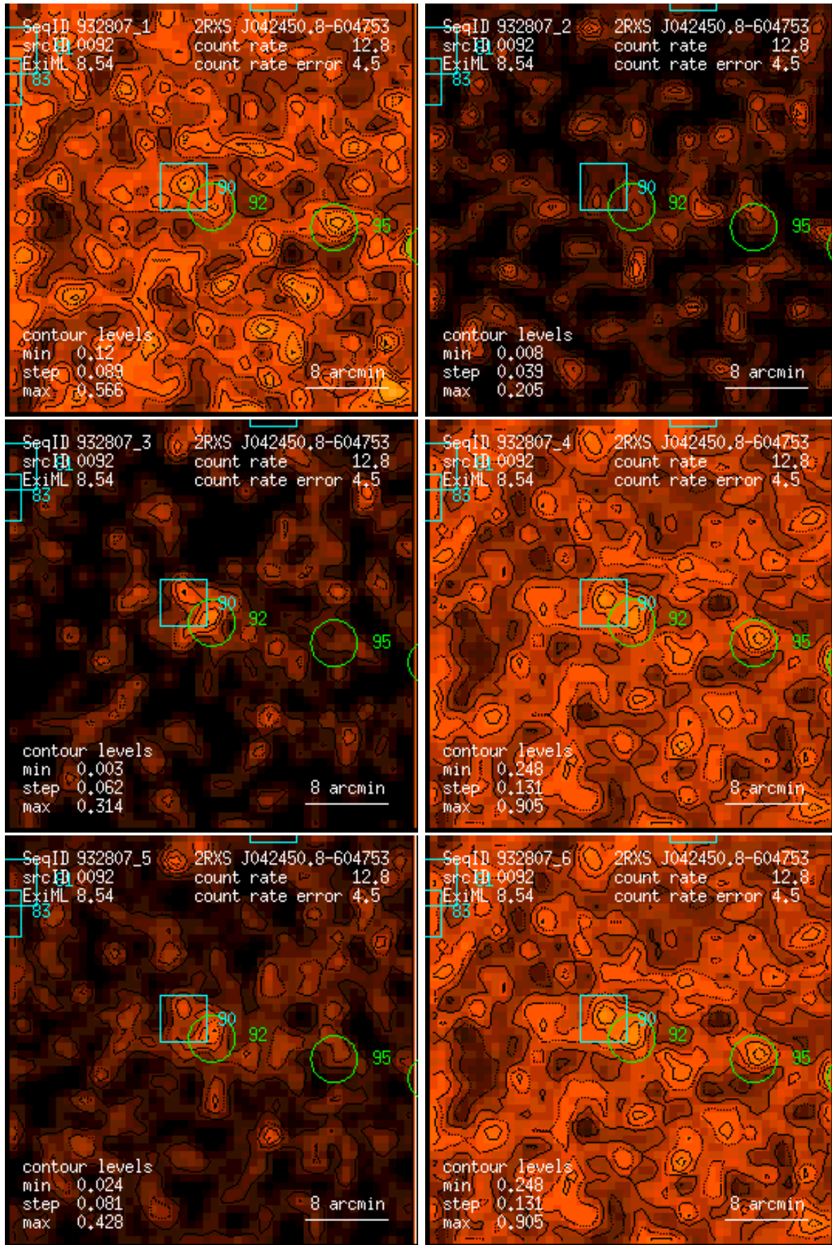
Figure 92: RASS 932807: detection 0092: band rate images, Gaussian filter: (1) PSPC channels 11 – 41, (2) 52 – 90, (3) 91 – 201, (4) 11 – 235, (5) 52 – 201, (6) 11 – 201. Broad band rates in counts/ks. Band rate contour levels in counts/ks/arcmin 2 .
