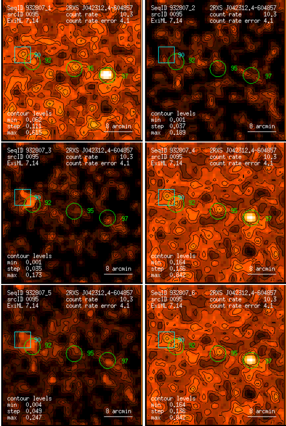
Figure 95: RASS 932807: detection 0095: band rate images, Gaussian filter: (1) PSPC channels 11 – 41, (2) 52 – 90, (3) 91 – 201, (4) 11 – 235, (5) 52 – 201, (6) 11 – 201. Broad band rates in counts/ks. Band rate contour levels in counts/ks/arcmin 2 .
