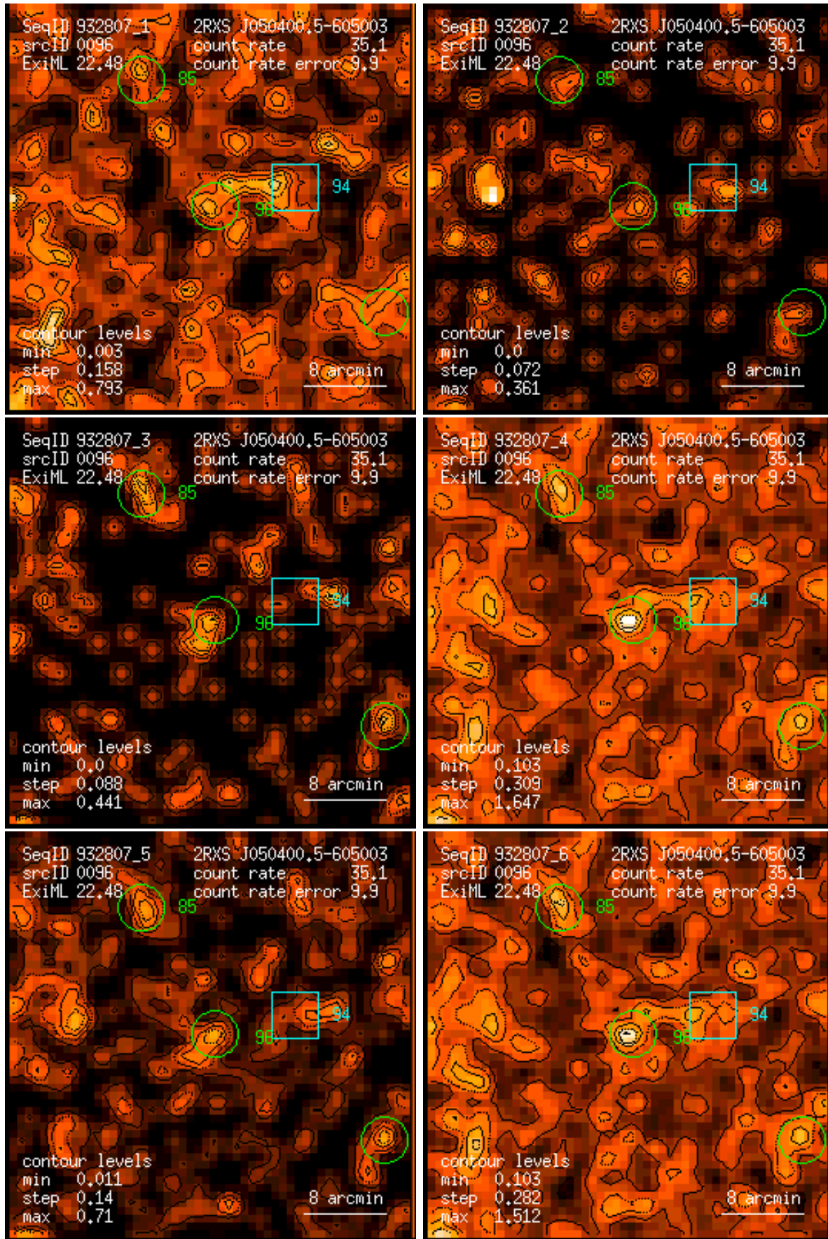
Figure 96: RASS 932807: detection 0096: band rate images, Gaussian filter: (1) PSPC channels 11 – 41, (2) 52 – 90, (3) 91 – 201, (4) 11 – 235, (5) 52 – 201, (6) 11 – 201. Broad band rates in counts/ks. Band rate contour levels in counts/ks/arcmin 2 .
