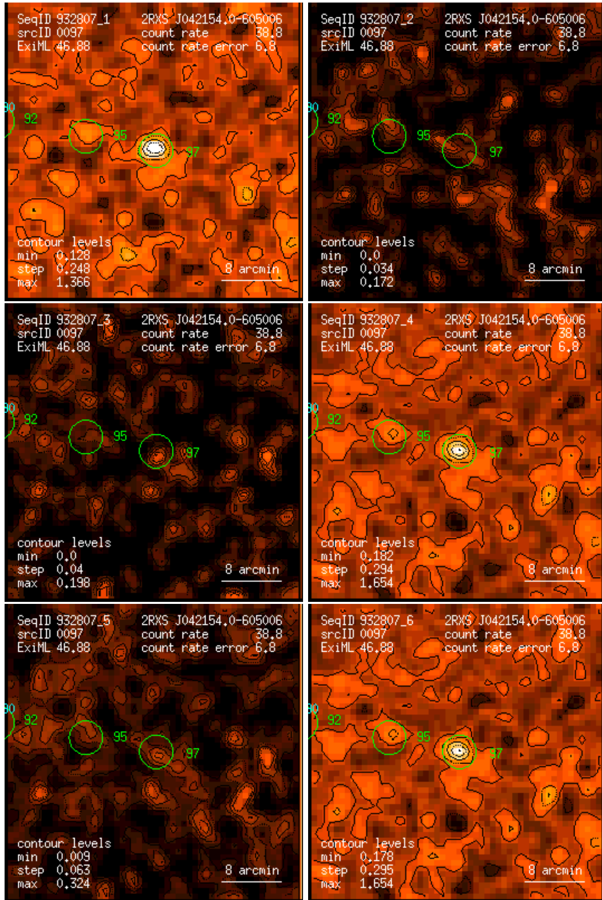
Figure 97: RASS 932807: detection 0097: band rate images, Gaussian filter: (1) PSPC channels 11 – 41, (2) 52 – 90, (3) 91 – 201, (4) 11 – 235, (5) 52 – 201, (6) 11 – 201. Broad band rates in counts/ks. Band rate contour levels in counts/ks/arcmin 2 .
