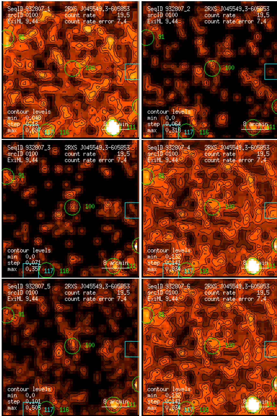
Figure 100: RASS 932807: detection 0100: band rate images, Gaussian filter: (1) PSPC channels 11 – 41, (2) 52 – 90, (3) 91 – 201, (4) 11 – 235, (5) 52 – 201, (6) 11 – 201. Broad band rates in counts/ks. Band rate contour levels in counts/ks/arcmin 2 .
