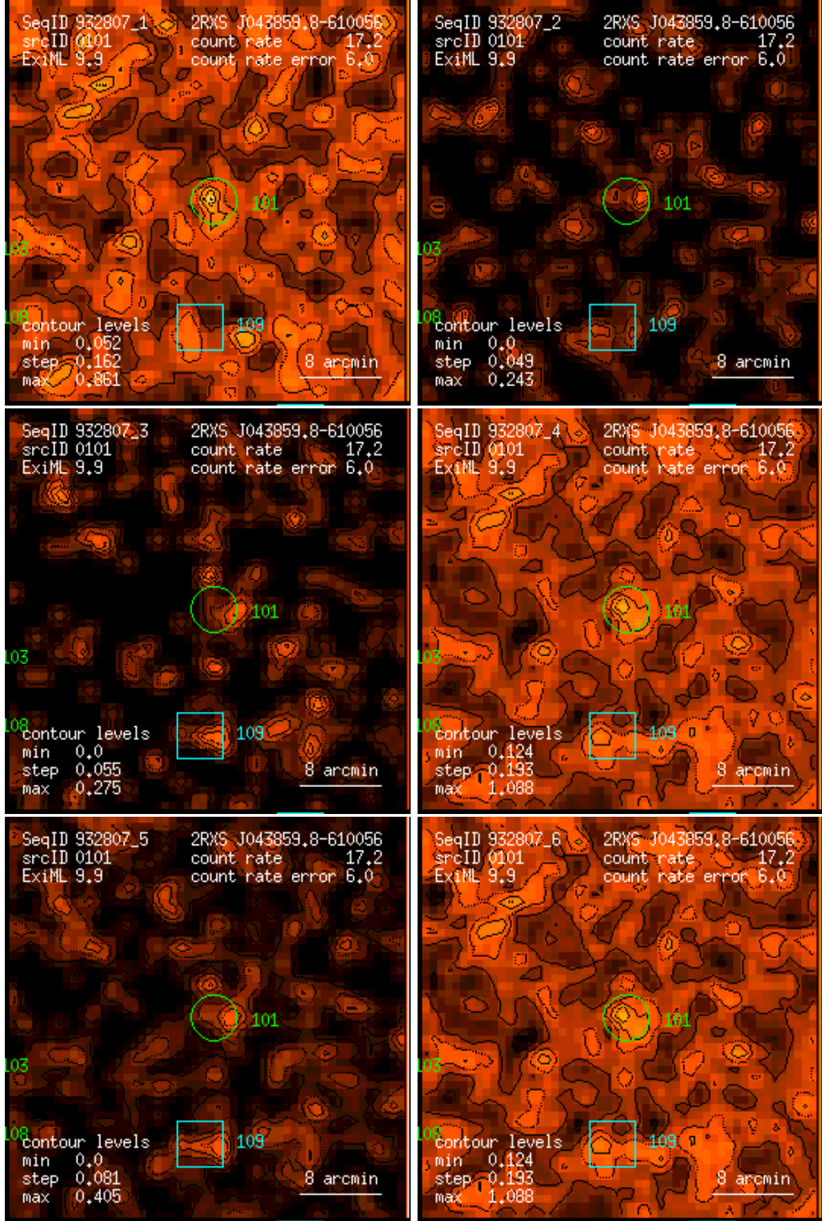
Figure 101: RASS 932807: detection 0101: band rate images, Gaussian filter: (1) PSPC channels 11 – 41, (2) 52 – 90, (3) 91 – 201, (4) 11 – 235, (5) 52 – 201, (6) 11 – 201. Broad band rates in counts/ks. Band rate contour levels in counts/ks/arcmin 2 .
