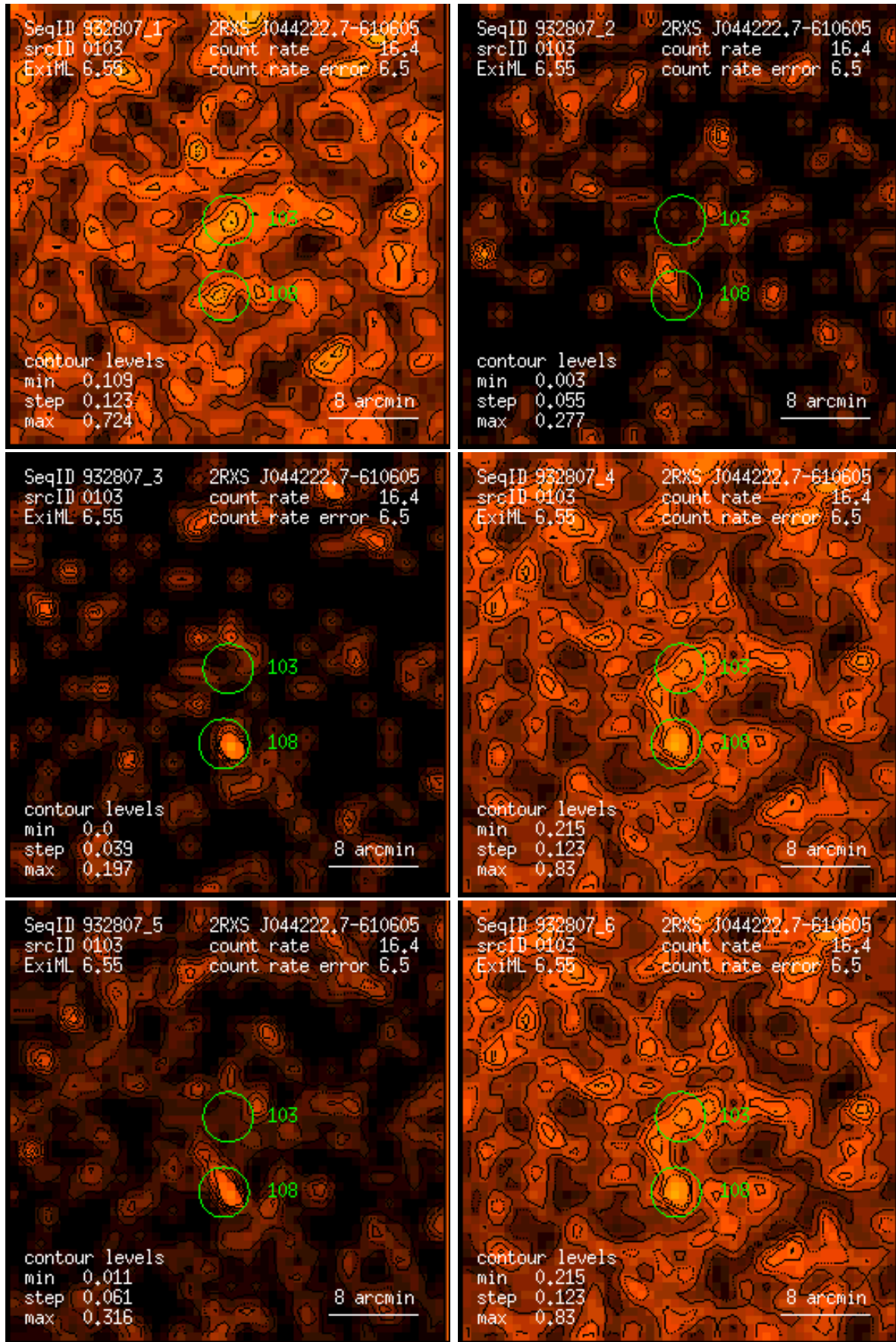
Figure 103: RASS 932807: detection 0103: band rate images, Gaussian filter: (1) PSPC channels 11 – 41, (2) 52 – 90, (3) 91 – 201, (4) 11 – 235, (5) 52 – 201, (6) 11 – 201. Broad band rates in counts/ks. Band rate contour levels in counts/ks/arcmin 2 .
