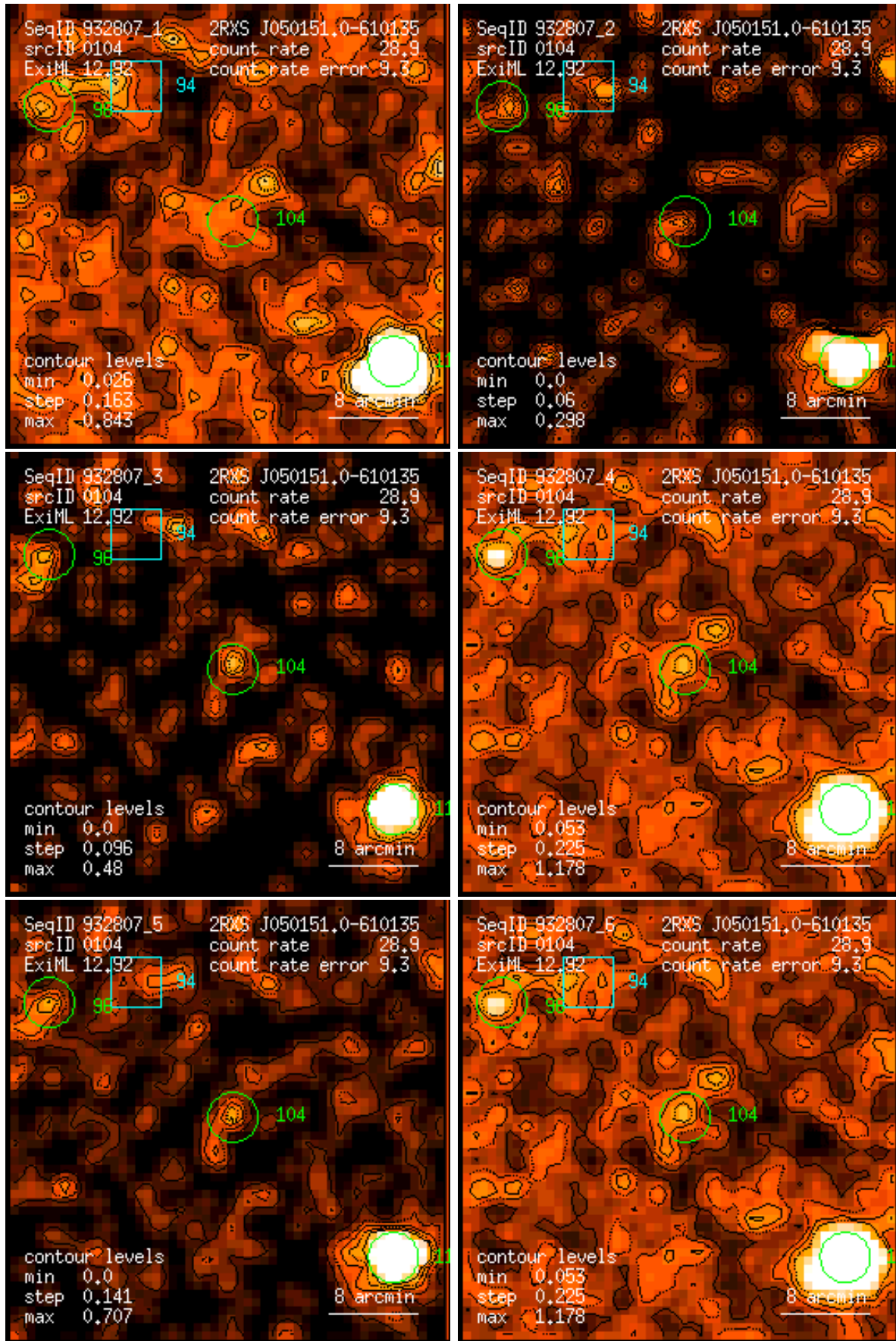
Figure 104: RASS 932807: detection 0104: band rate images, Gaussian filter: (1) PSPC channels 11 – 41, (2) 52 – 90, (3) 91 – 201, (4) 11 – 235, (5) 52 – 201, (6) 11 – 201. Broad band rates in counts/ks. Band rate contour levels in counts/ks/arcmin 2 .
