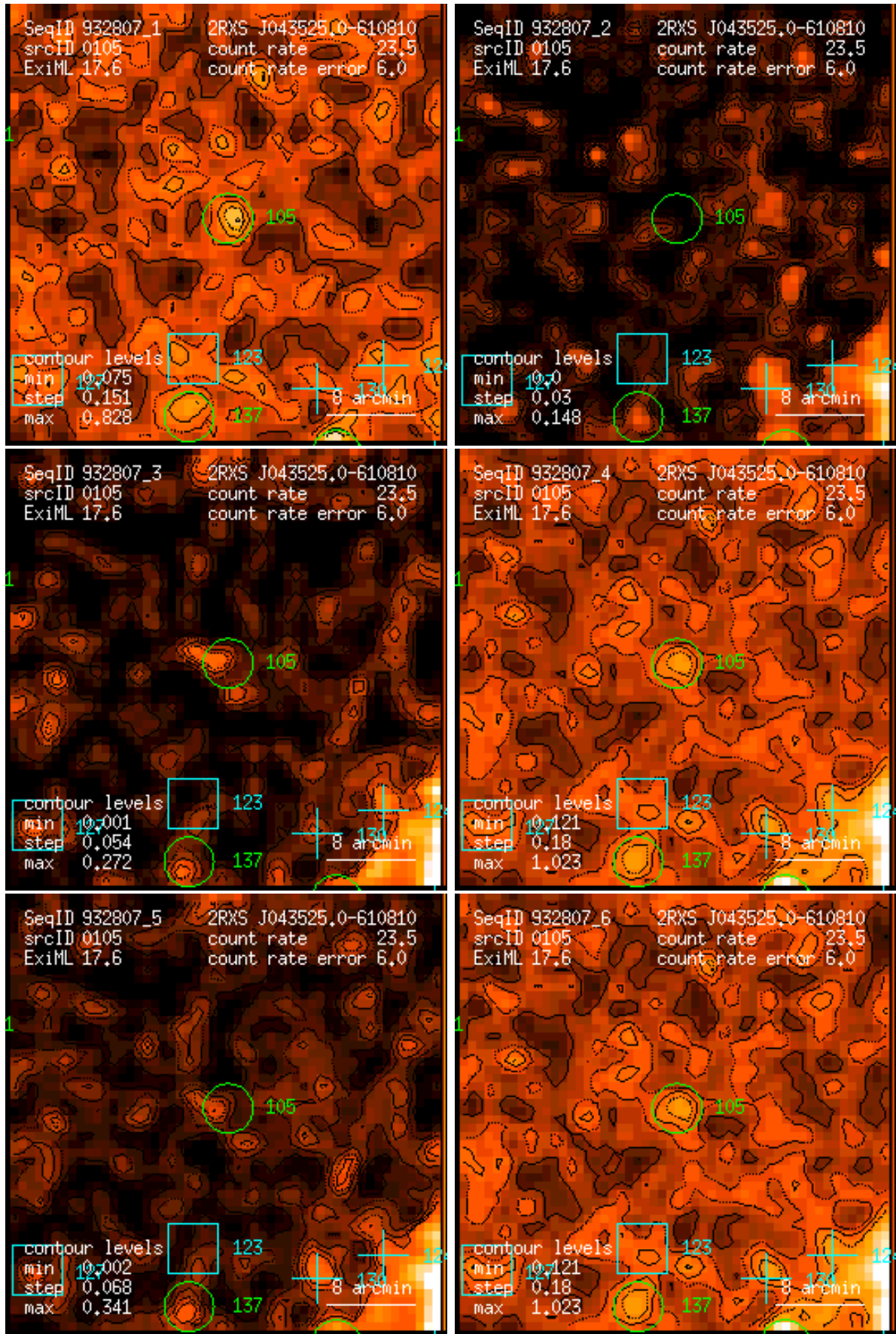
Figure 105: RASS 932807: detection 0105: band rate images, Gaussian filter: (1) PSPC channels 11 – 41, (2) 52 – 90, (3) 91 – 201, (4) 11 – 235, (5) 52 – 201, (6) 11 – 201. Broad band rates in counts/ks. Band rate contour levels in counts/ks/arcmin 2 .
