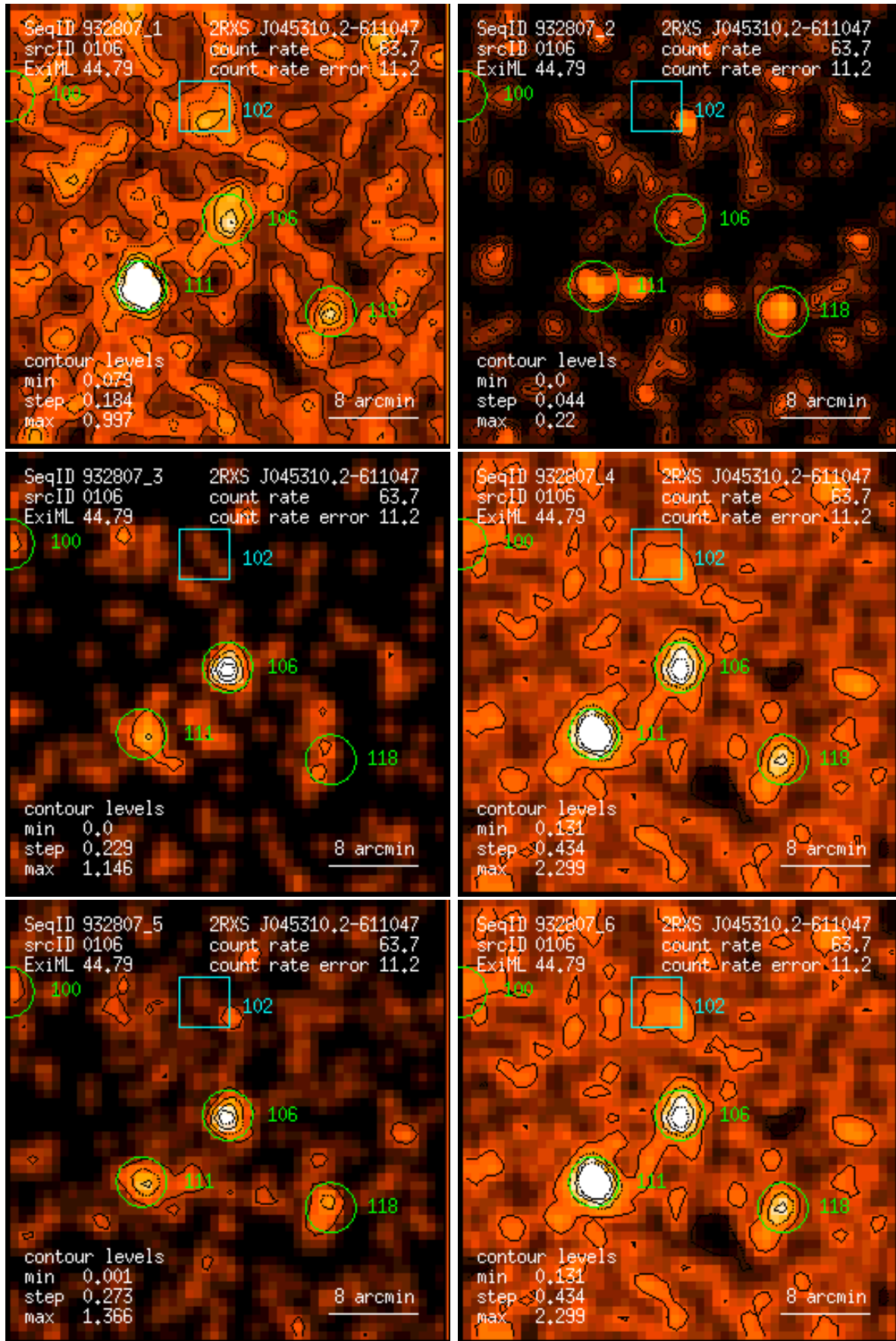
Figure 106: RASS 932807: detection 0106: band rate images, Gaussian filter: (1) PSPC channels 11 – 41, (2) 52 – 90, (3) 91 – 201, (4) 11 – 235, (5) 52 – 201, (6) 11 – 201. Broad band rates in counts/ks. Band rate contour levels in counts/ks/arcmin 2 .
