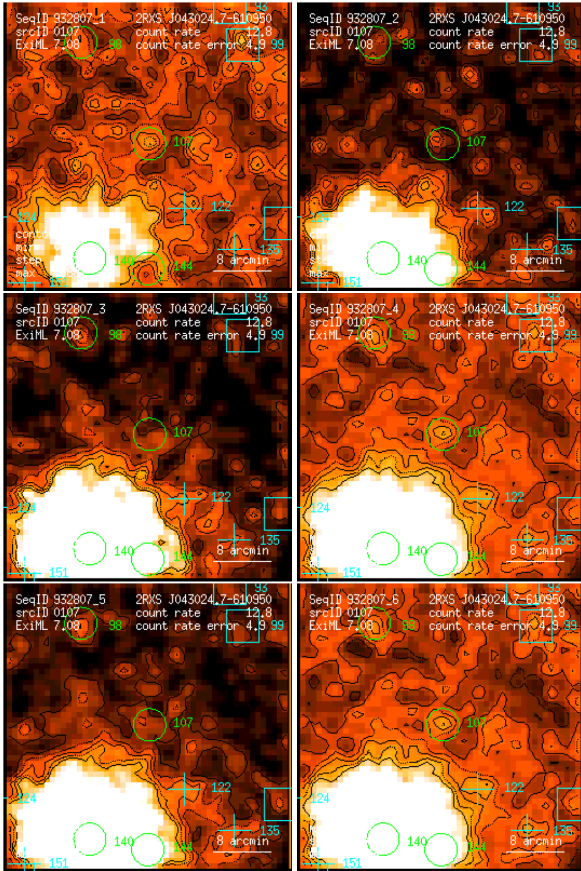
Figure 107: RASS 932807: detection 0107: band rate images, Gaussian filter: (1) PSPC channels 11 – 41, (2) 52 – 90, (3) 91 – 201, (4) 11 – 235, (5) 52 – 201, (6) 11 – 201. Broad band rates in counts/ks. Band rate contour levels in counts/ks/arcmin 2 .
