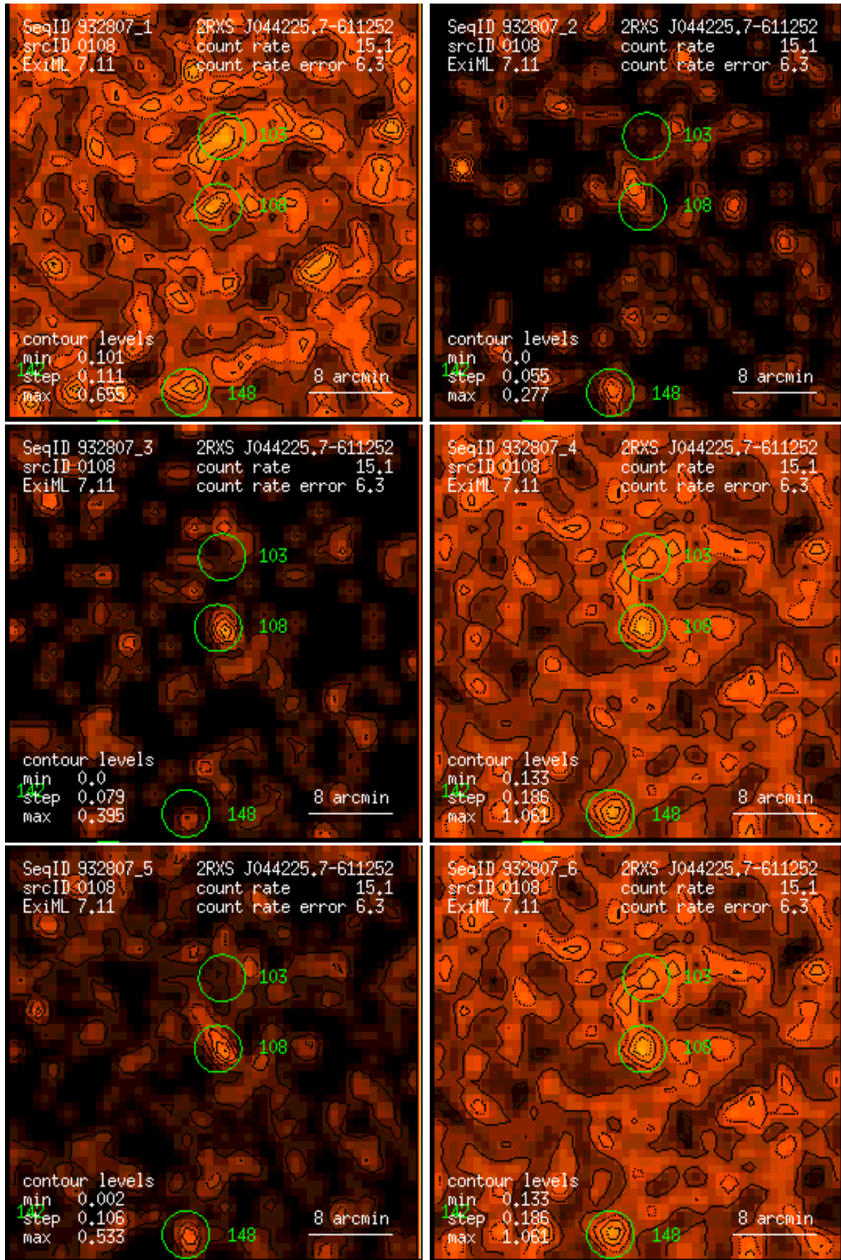
Figure 108: RASS 932807: detection 0108: band rate images, Gaussian filter: (1) PSPC channels 11 – 41, (2) 52 – 90, (3) 91 – 201, (4) 11 – 235, (5) 52 – 201, (6) 11 – 201. Broad band rates in counts/ks. Band rate contour levels in counts/ks/arcmin 2 .
