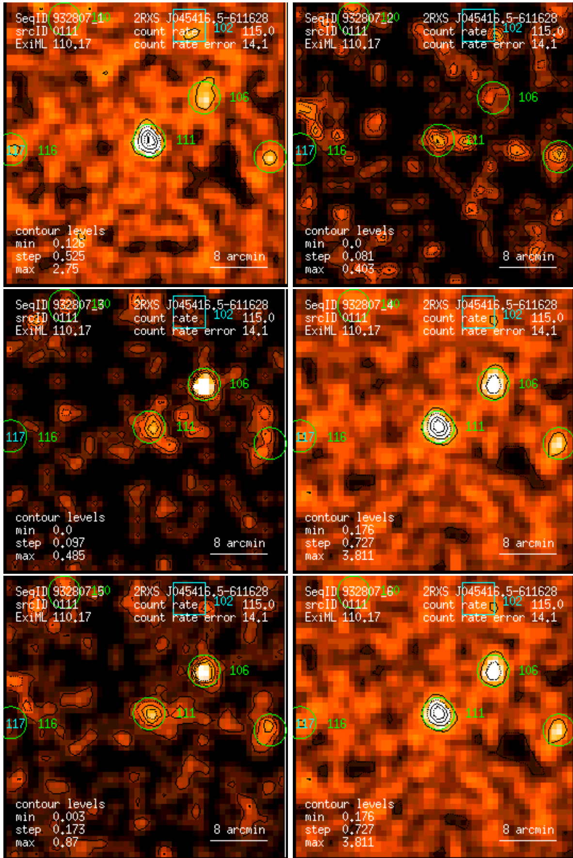
Figure 111: RASS 932807: detection 0111: band rate images, Gaussian filter: (1) PSPC channels 11 – 41, (2) 52 – 90, (3) 91 – 201, (4) 11 – 235, (5) 52 – 201, (6) 11 – 201. Broad band rates in counts/ks. Band rate contour levels in counts/ks/arcmin 2 .
