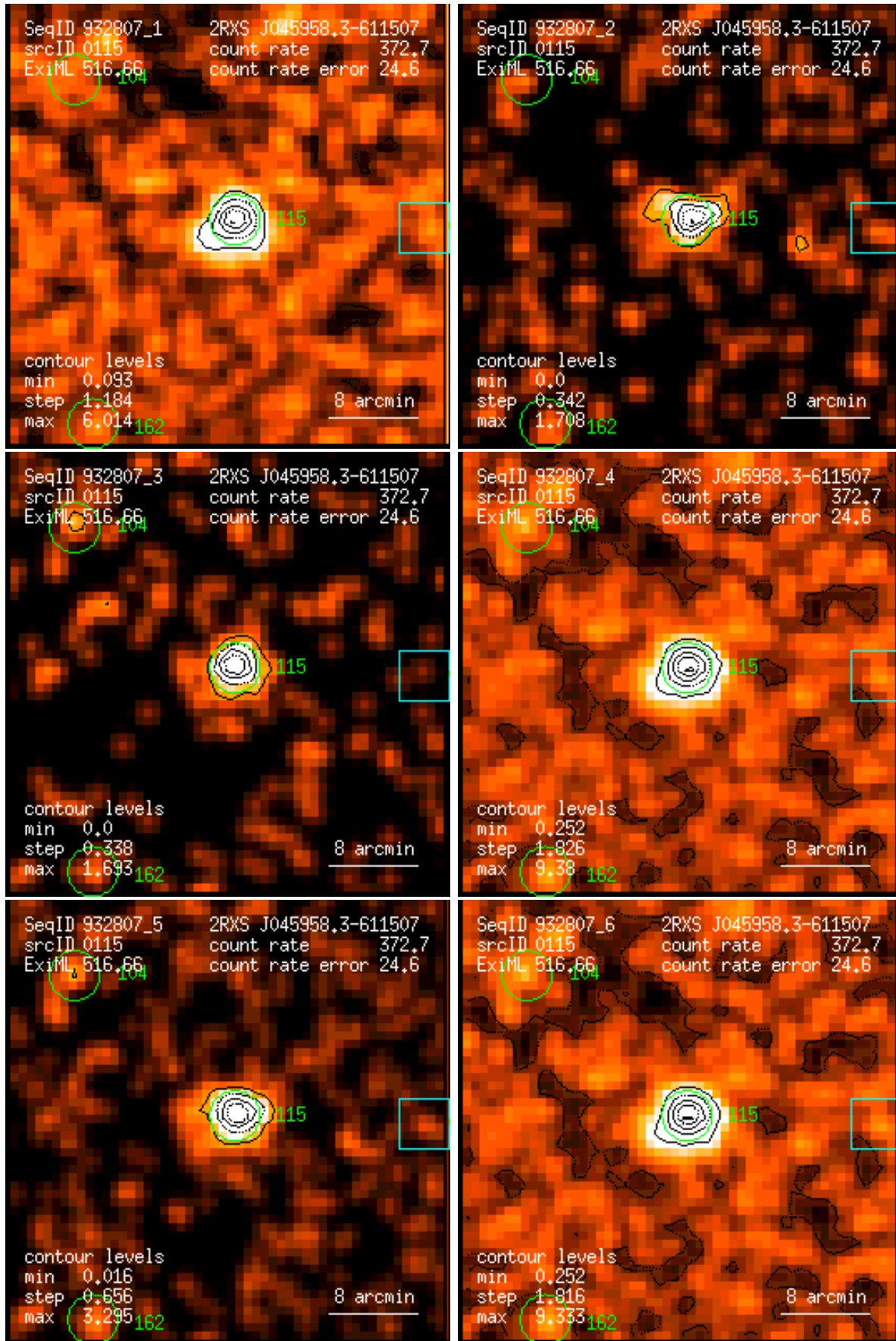
Figure 115: RASS 932807: detection 0115: band rate images, Gaussian filter: (1) PSPC channels 11 – 41, (2) 52 – 90, (3) 91 – 201, (4) 11 – 235, (5) 52 – 201, (6) 11 – 201. Broad band rates in counts/ks. Band rate contour levels in counts/ks/arcmin 2 .
