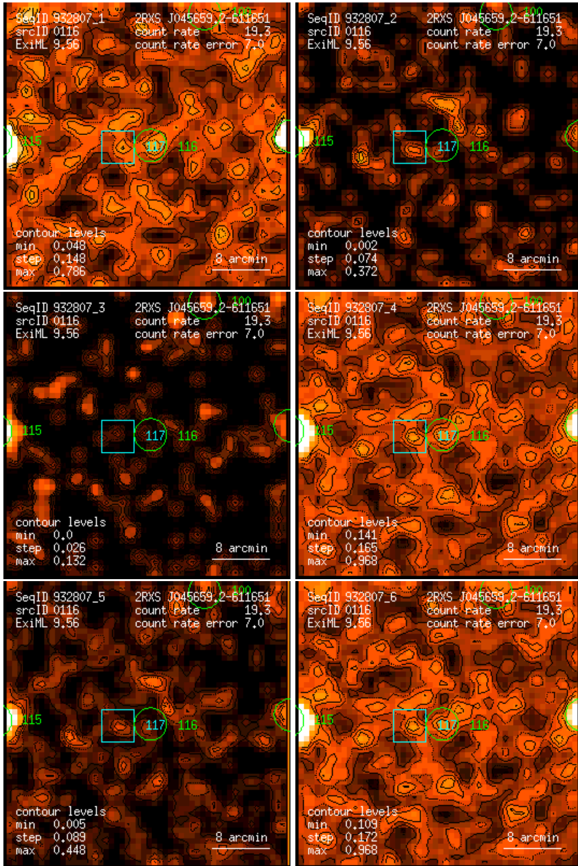
Figure 116: RASS 932807: detection 0116: band rate images, Gaussian filter: (1) PSPC channels 11 – 41, (2) 52 – 90, (3) 91 – 201, (4) 11 – 235, (5) 52 – 201, (6) 11 – 201. Broad band rates in counts/ks. Band rate contour levels in counts/ks/arcmin 2 .
